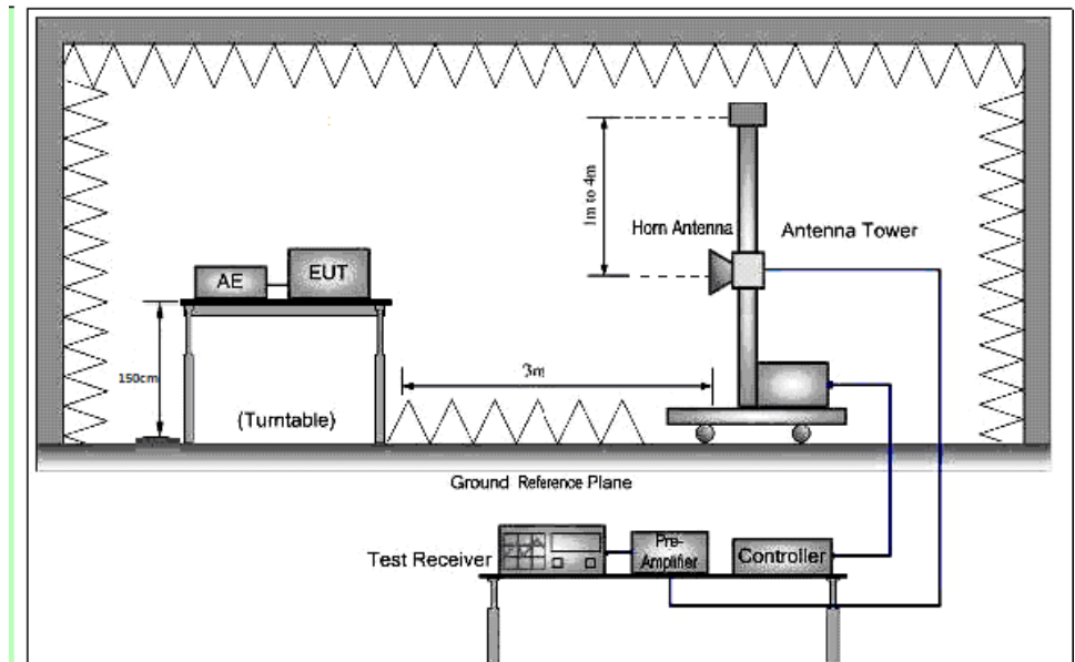
Above 1 GHz
