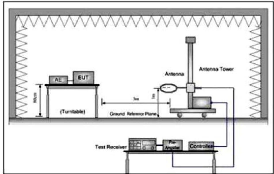
Below 30MHz
