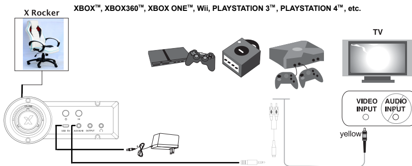
DIAGRAM 1 GAMING SYSTEMS
