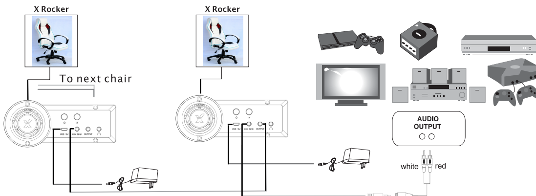
DIAGRAM 4 MULTI-USER CONNECTION
