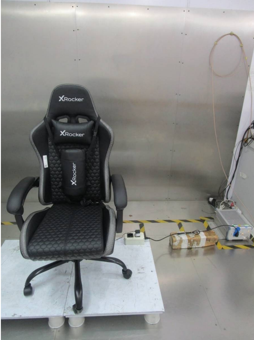
Conducted Emissions at AC Power Line (150kHz-30MHz)
