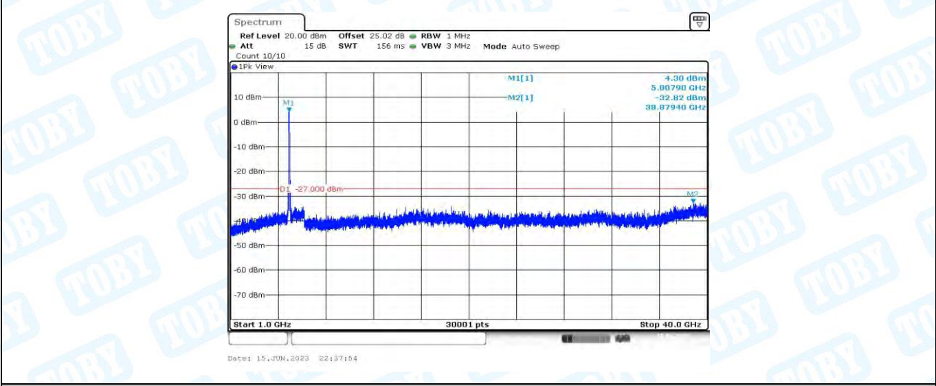
11AC80MIMO_Ant1_5775_1000~40000
