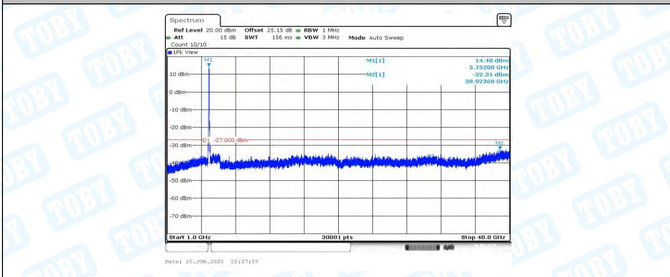
11AC40MIMO_Ant1_5755_1000~40000
