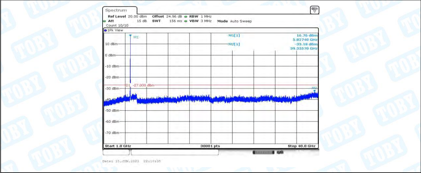
11AC20MIMO_Ant1_5825_1000~40000
