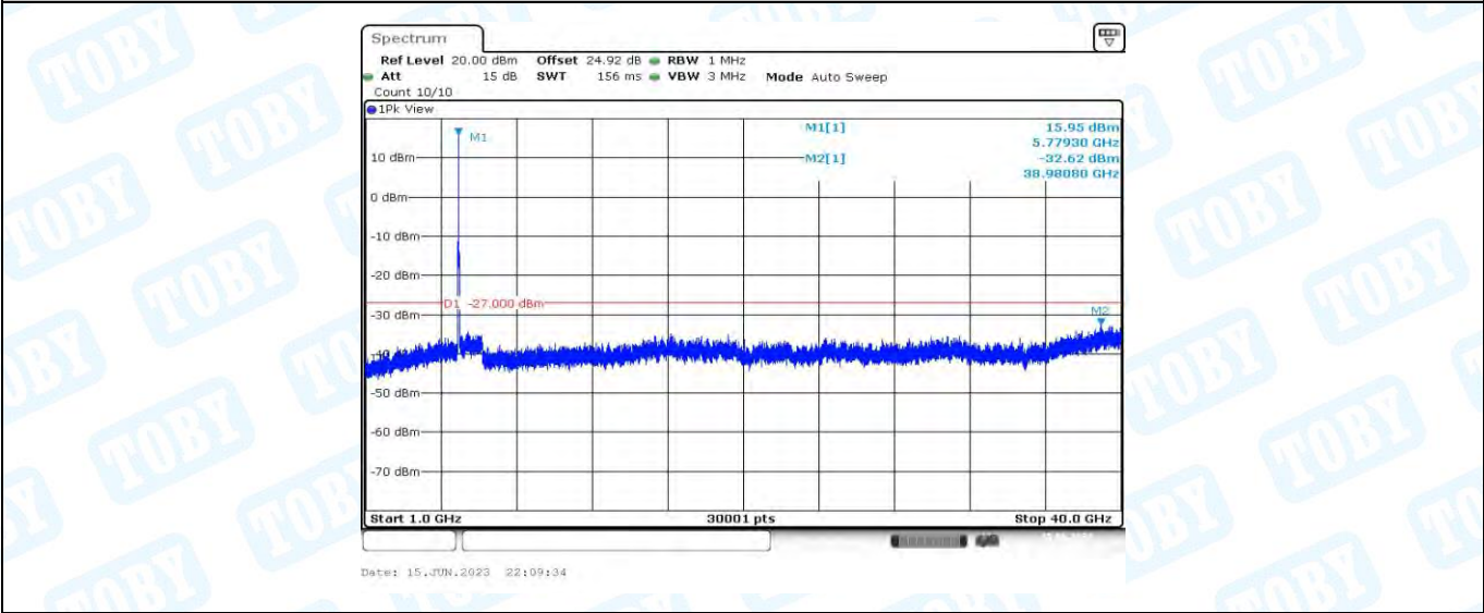
11AC20MIMO_Ant1_5785_1000~40000
