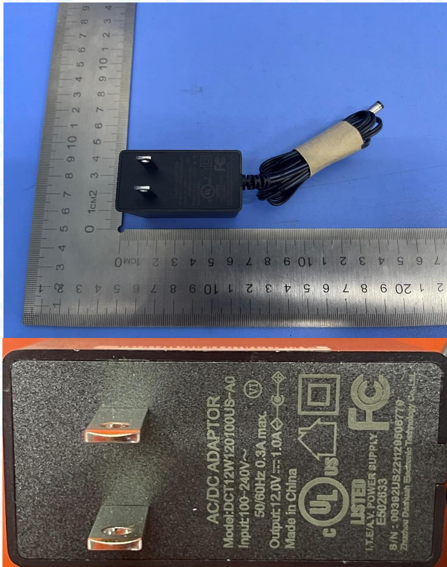
Photo 9 Appearance of Adapter 2# (DCT12W120100US-A0 DACHUAN)
