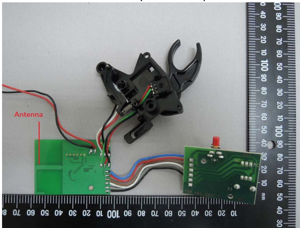
Antenna (Model: 6516B)
