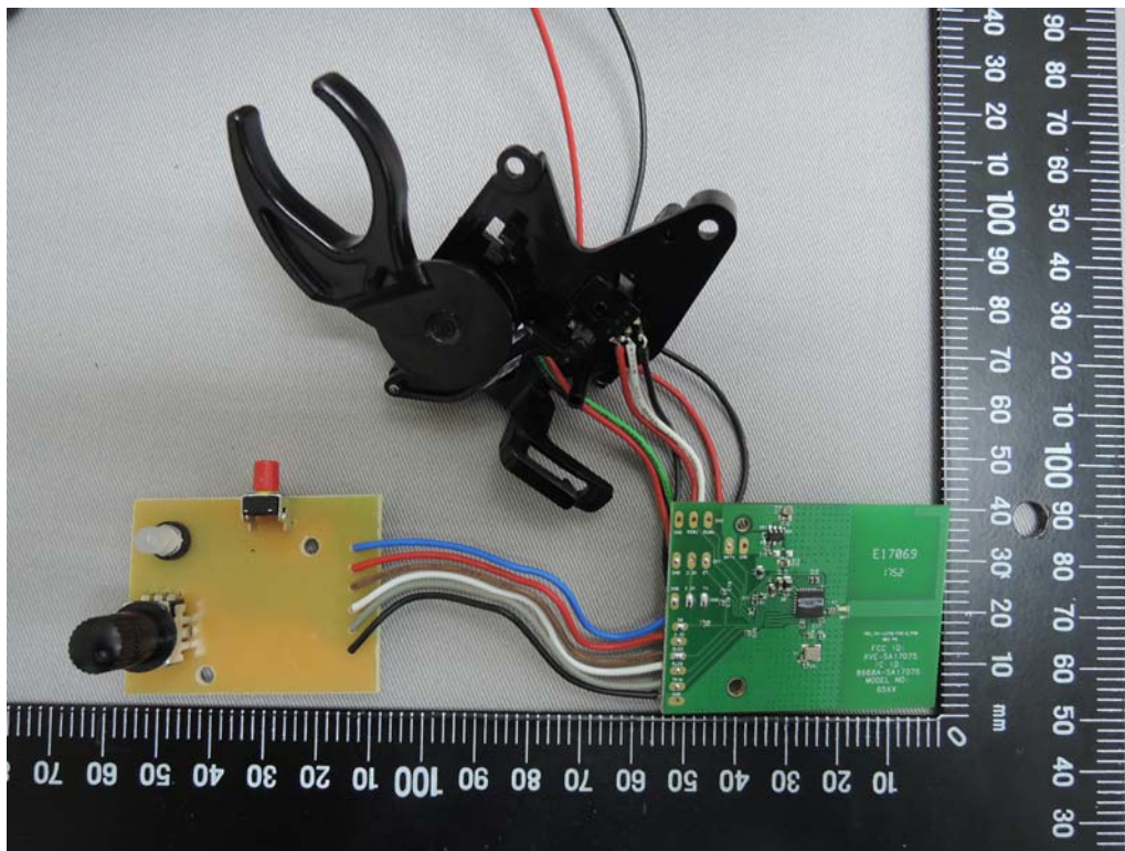
Internal View of EUT (Model: 3047B)
