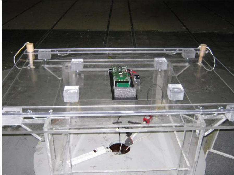
Radiated Emission (rear)
