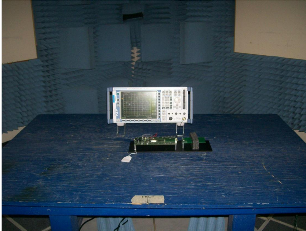
Conducted Emission
