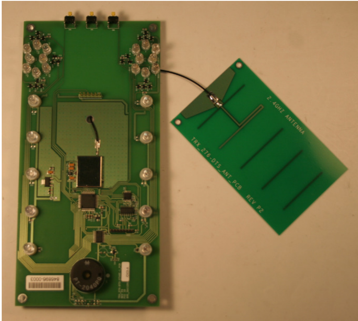
Figure 3 2.4GHz Transceiver Top with RF can
