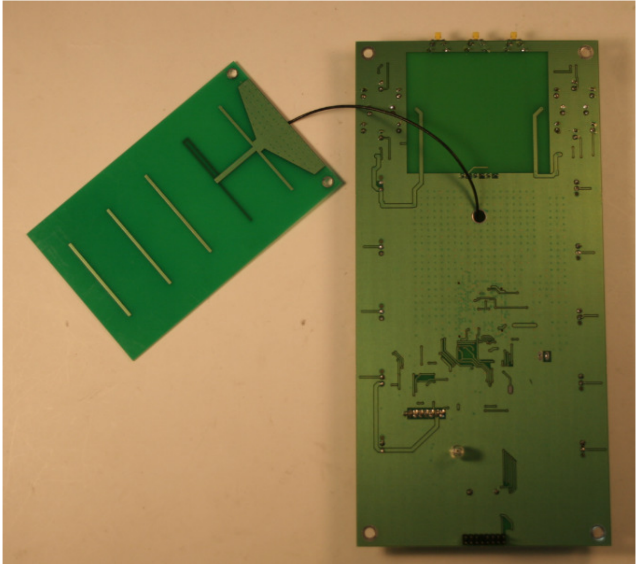
Figure 2 2.4GHz Transceiver Bottom
