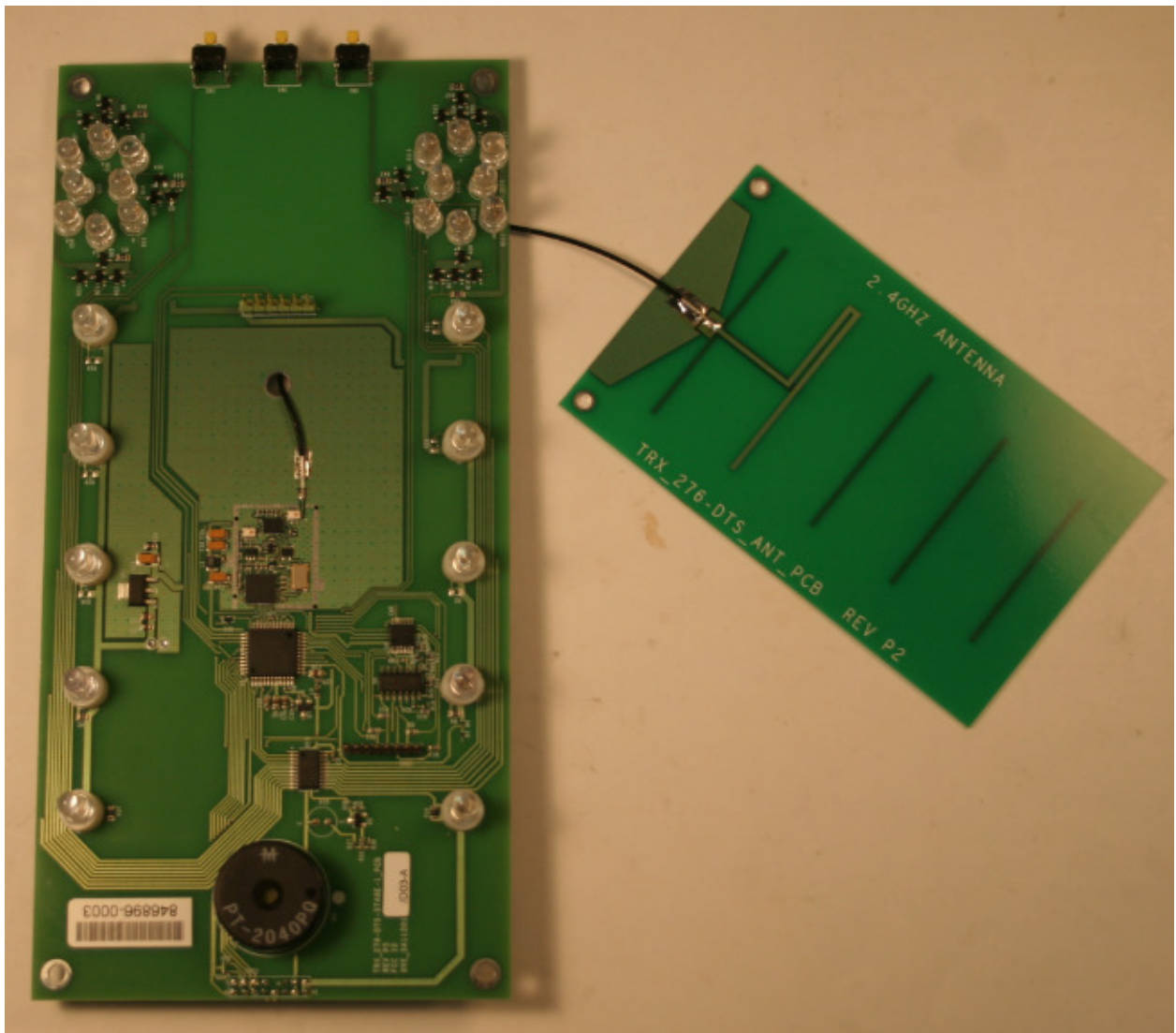
Figure 1 2.4GHz Transceiver Top
