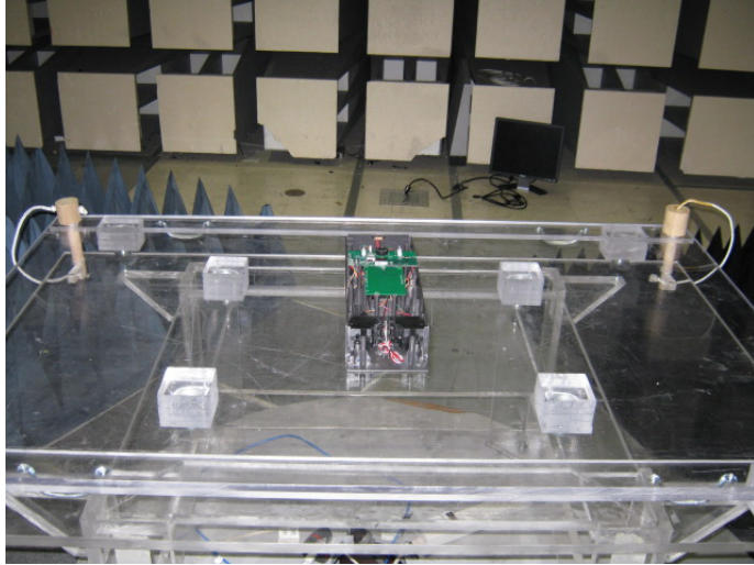
Radiated Emission
