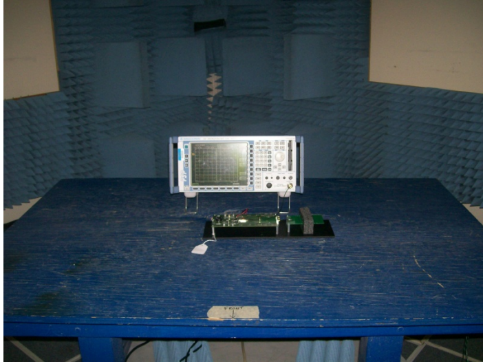
Conducted Emission Set up
