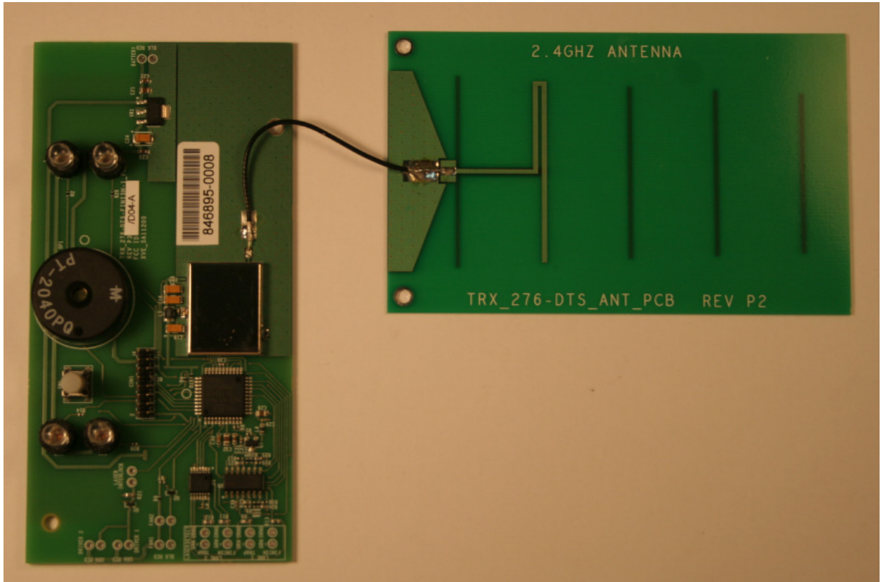
Figure 3 2.4GHz Transceiver Top with RF can
