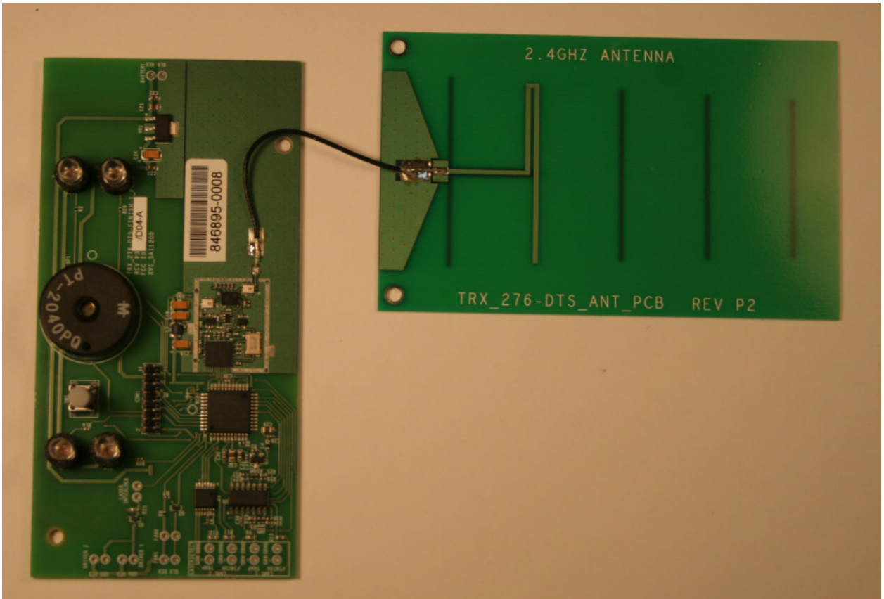
Figure 1 2.4GHz Transceiver Top
