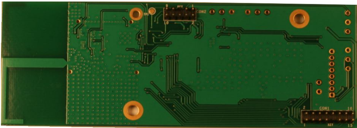
Figure 2 2.4GHz Transceiver Bottom
