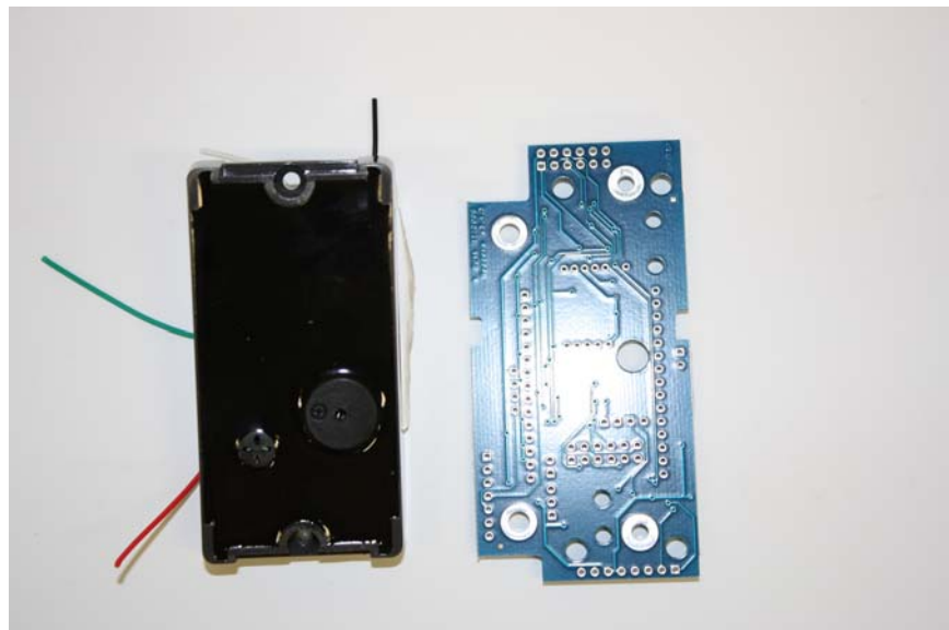
HID Prox Radio Module – Bottom View
