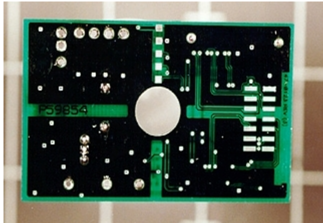
HID Global Internal – Bottom View
