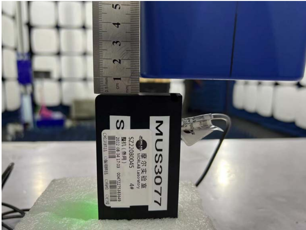
Left Side_10mm
