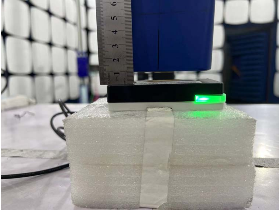
Front Side_10mm
