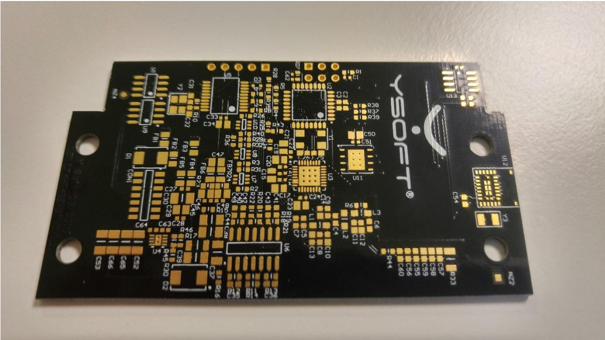
Reader PCB front not soldered
