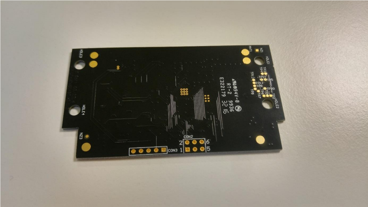
Reader PCB back
