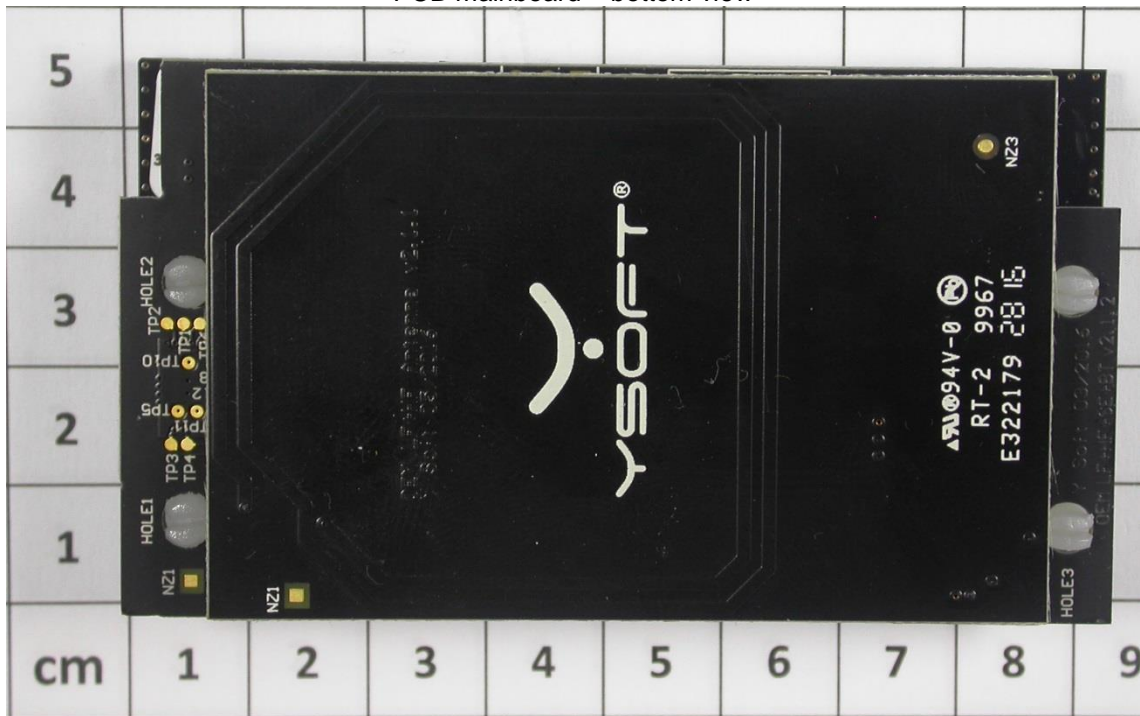
PCB mainboard – bottom view
