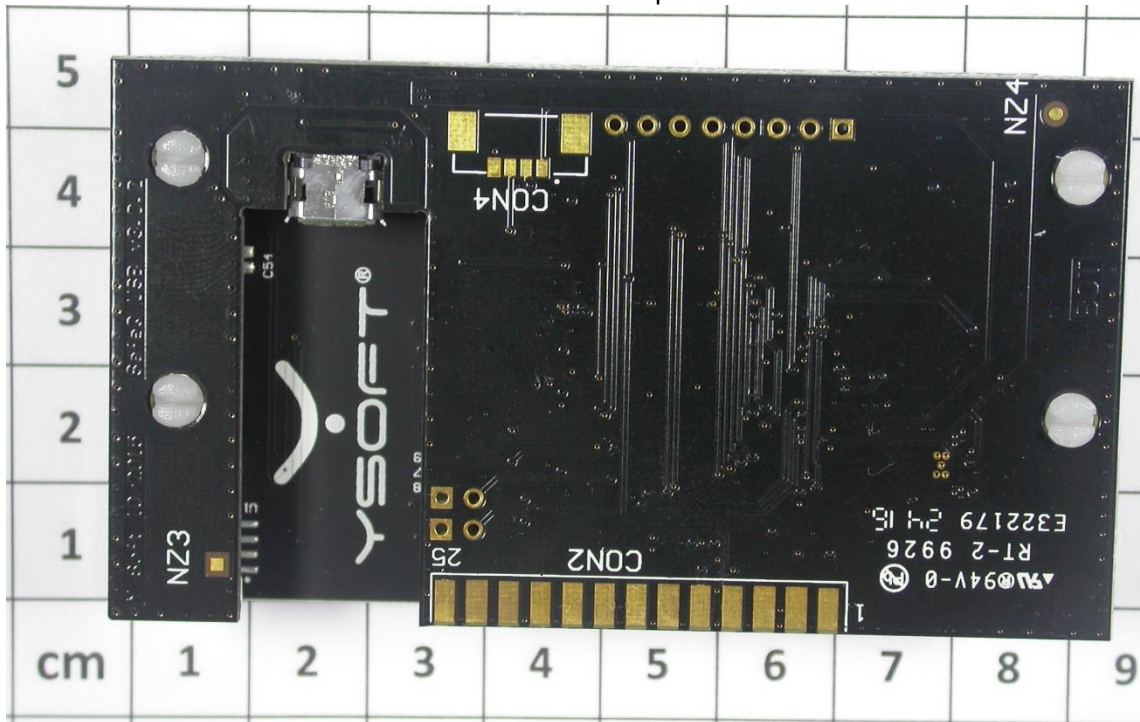
PCB mainboard – top view
