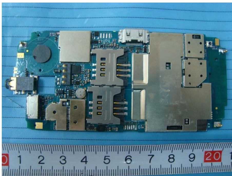
EUT – Main Board with shield Top View
