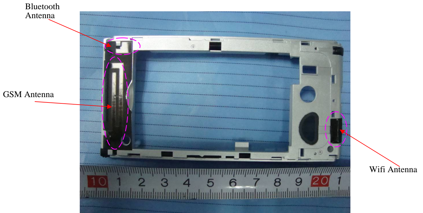
EUT – Antenna View
