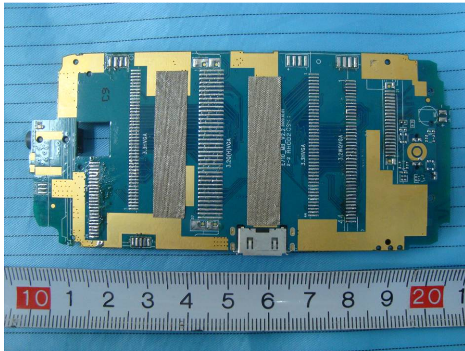
EUT – Main Board Bottom Circuit View
