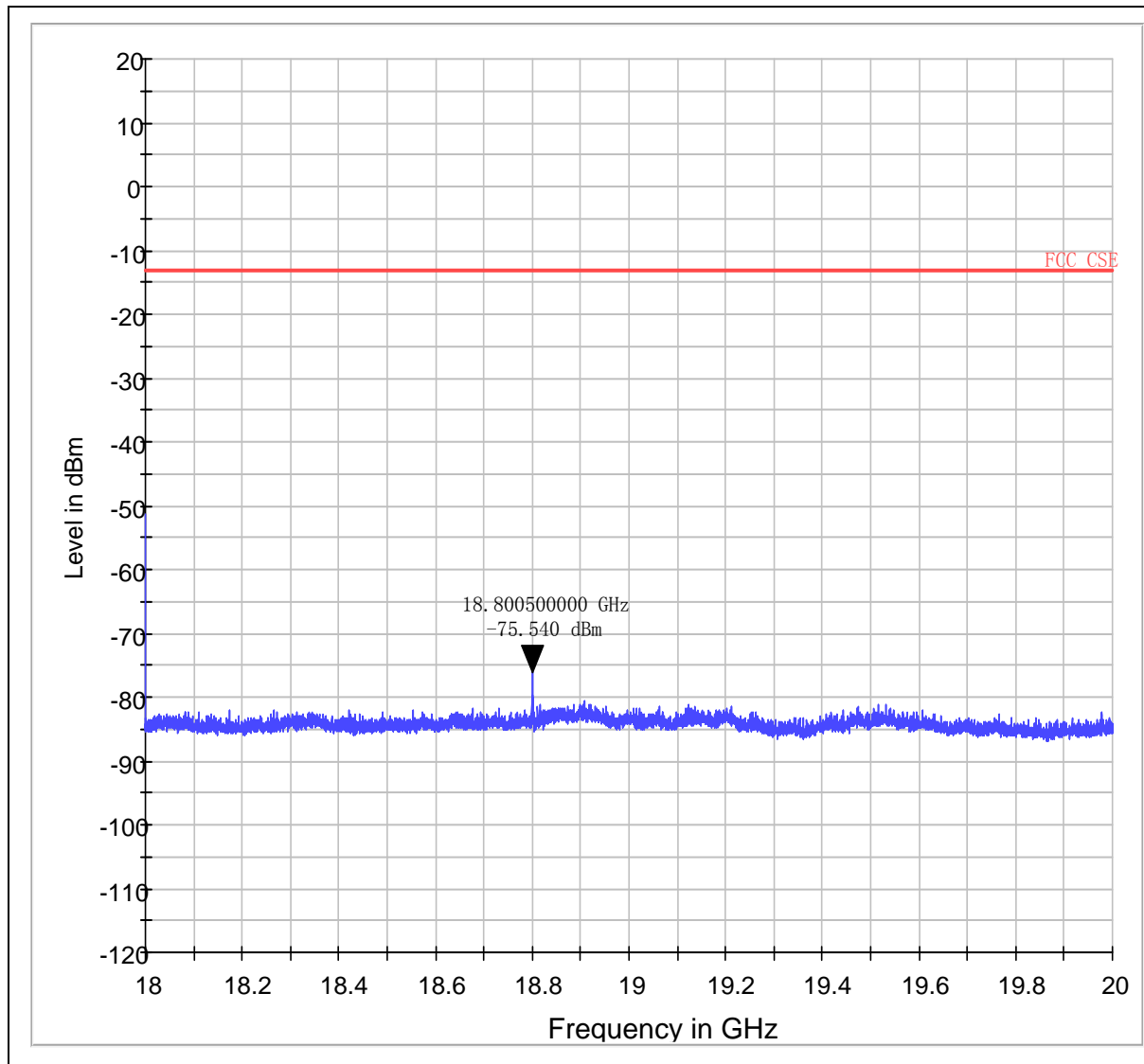
GSM 1900 661 Channel 18GHz ~20GHz
