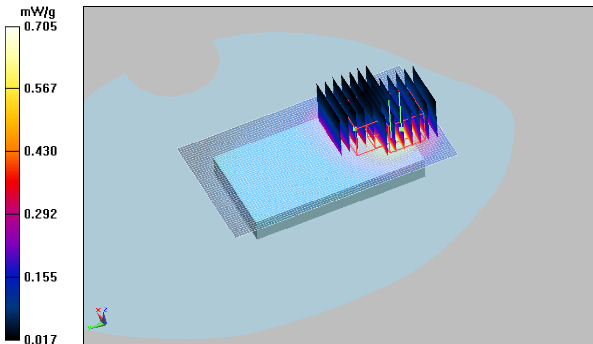
Figure 57 Body, Towards Ground, GSM 1900 GPRS(4up) Channel 810
