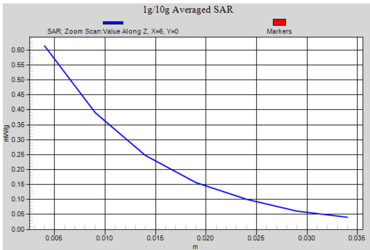
Figure 58 Z-Scan at power reference point (Body, Towards Ground, GSM 1900 GPRS(4up) Channel 810)
