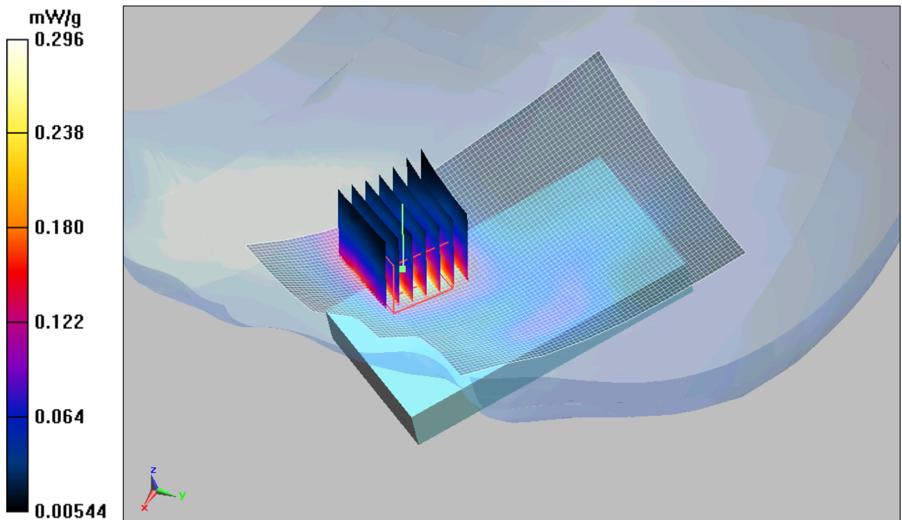
Figure 39 Left Hand Touch Cheek GSM 1900 Channel 661
