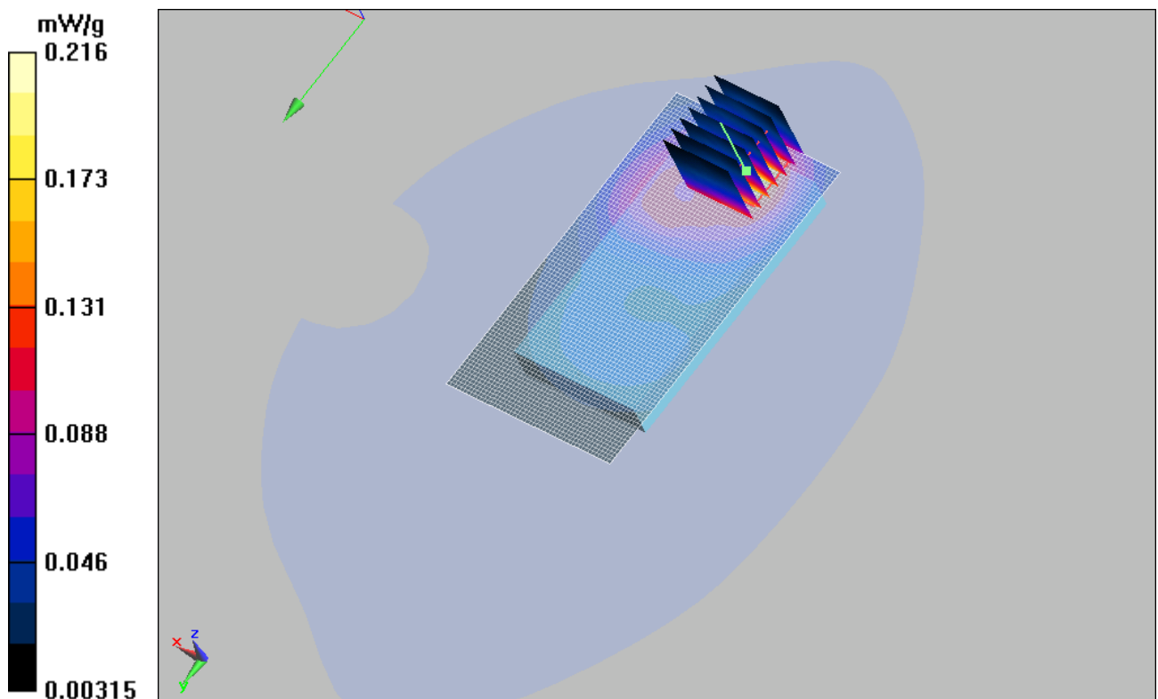
Figure 49 Body, Towards Ground, GSM 1900 Channel 810
