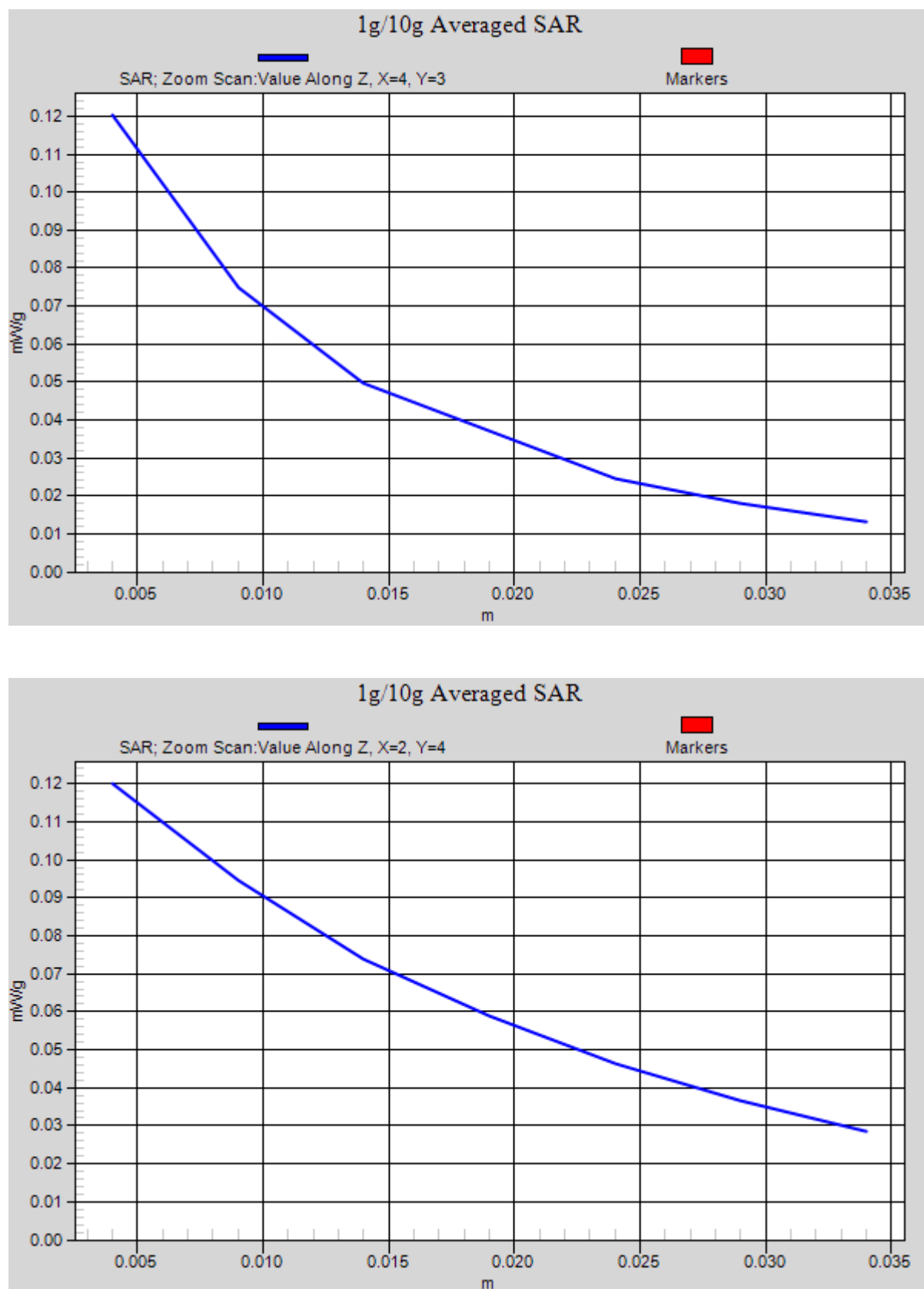
Figure 22 Z-Scan at power reference point (Left Hand Tilt 15° GSM 850 Channel 190)
