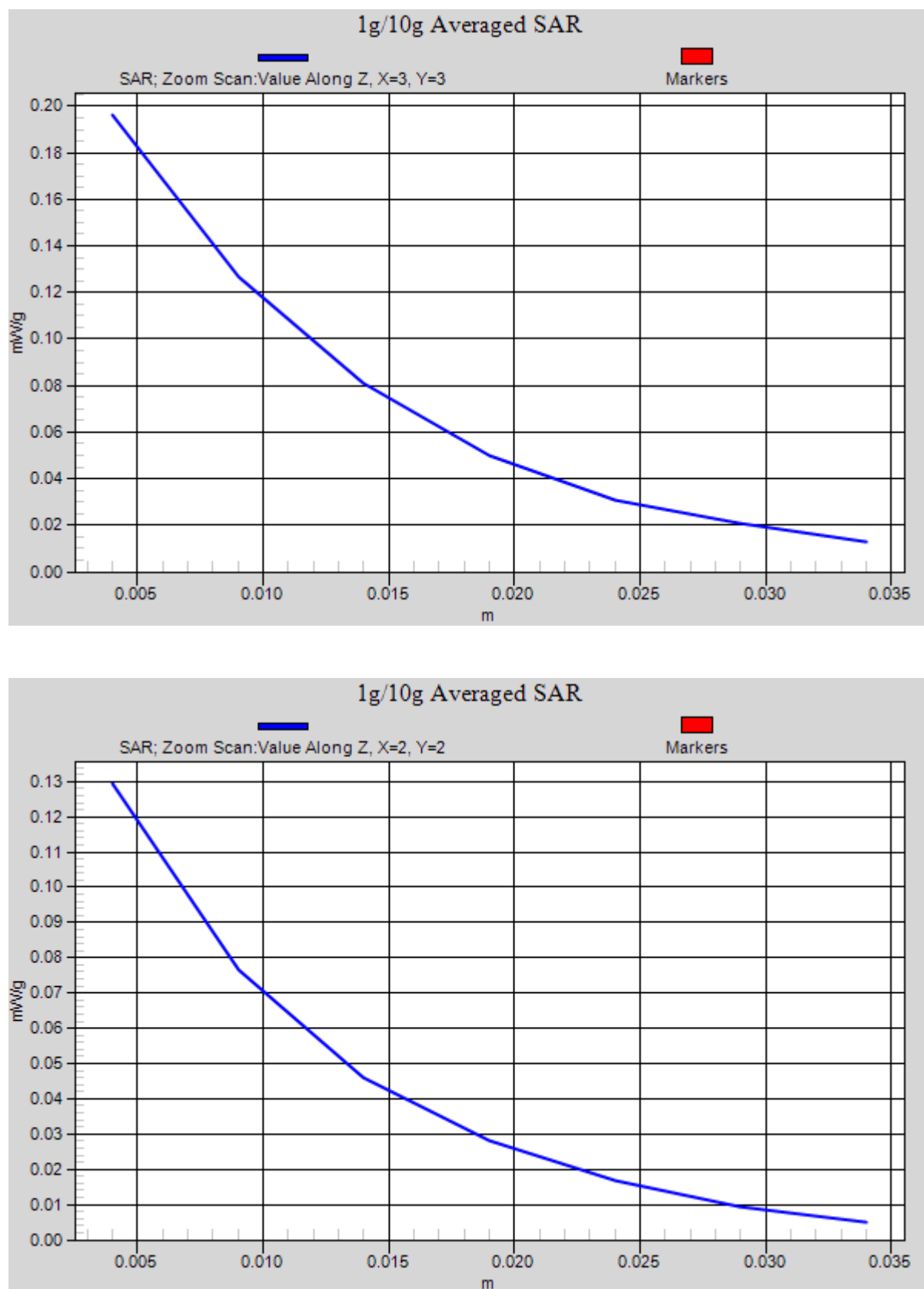
Figure 52 Z-Scan at power reference point (Body, Towards Ground, GSM 1900 Channel 661)
