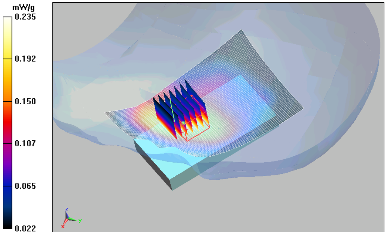
Figure 15 Left Hand Touch Cheek GSM 850 Channel 251
