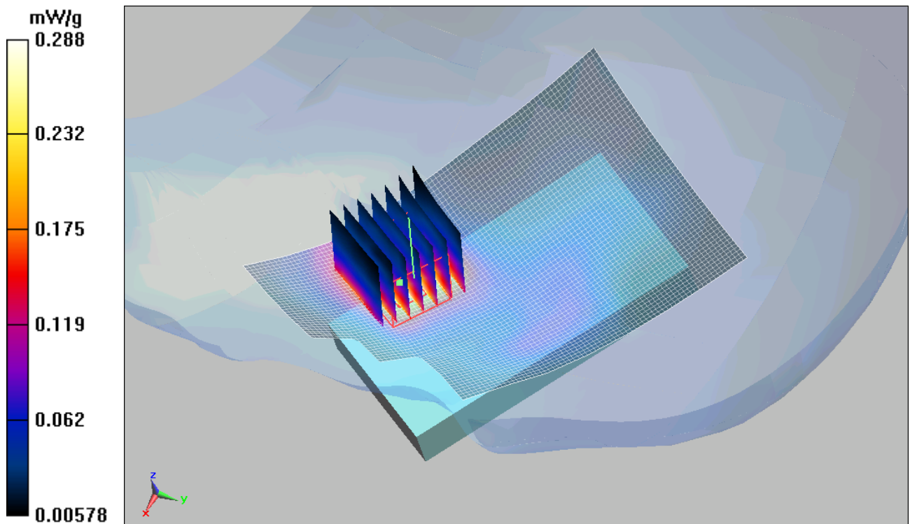
Figure 37 Left Hand Touch Cheek GSM 1900 Channel 810
