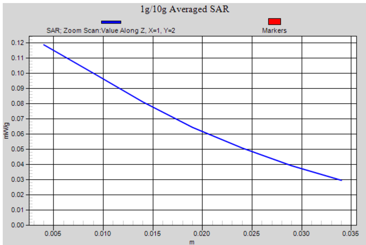
Figure 24 Z-Scan at power reference point (Right Hand Touch Cheek GSM 850 Channel 190)
