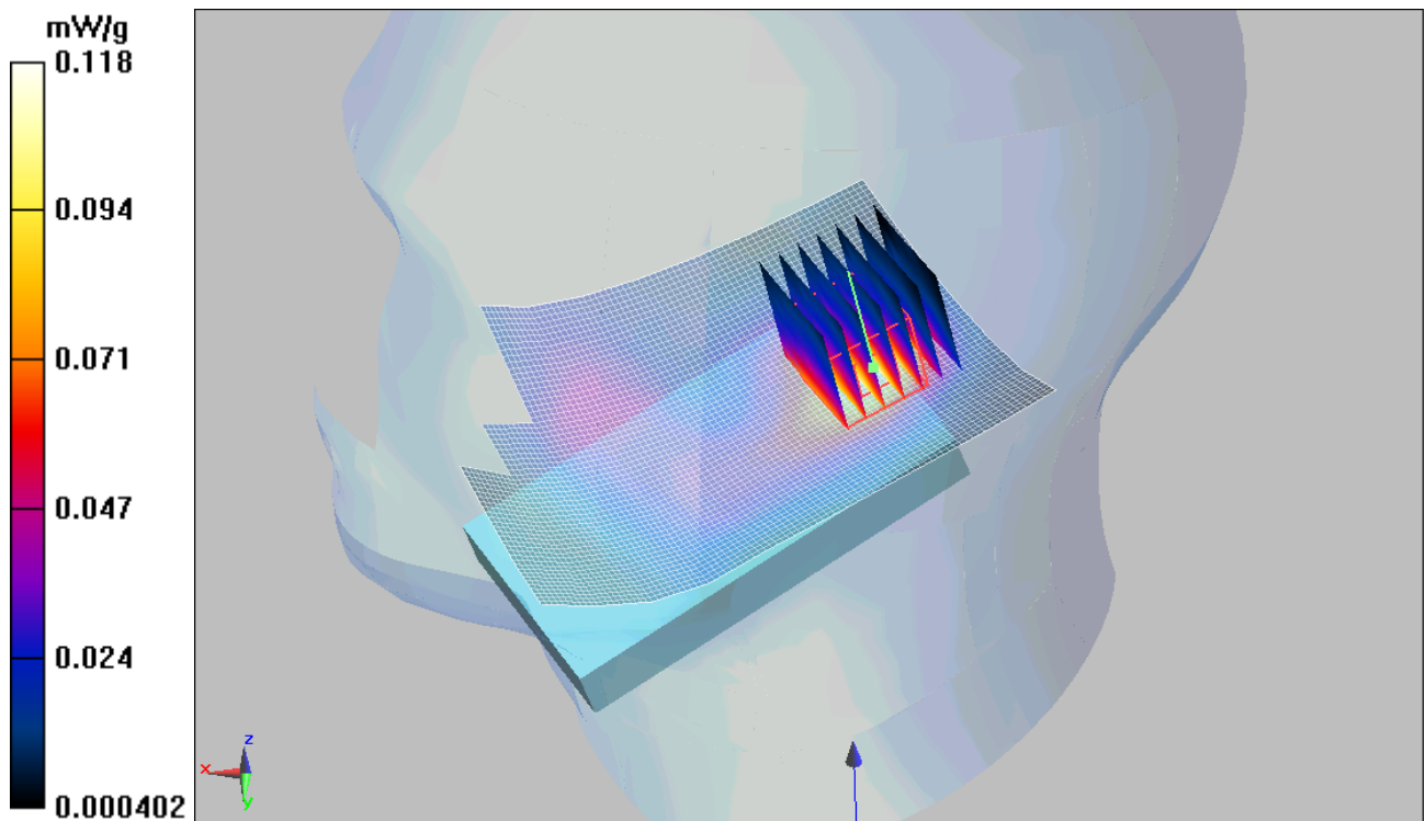
Figure 47 Right Hand Tilt 15° GSM 1900 Channel 661
