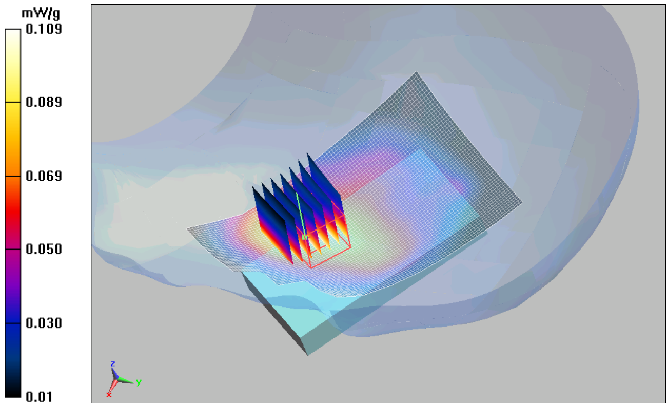
Figure 19 Left Hand Touch Cheek GSM 850 Channel 128
