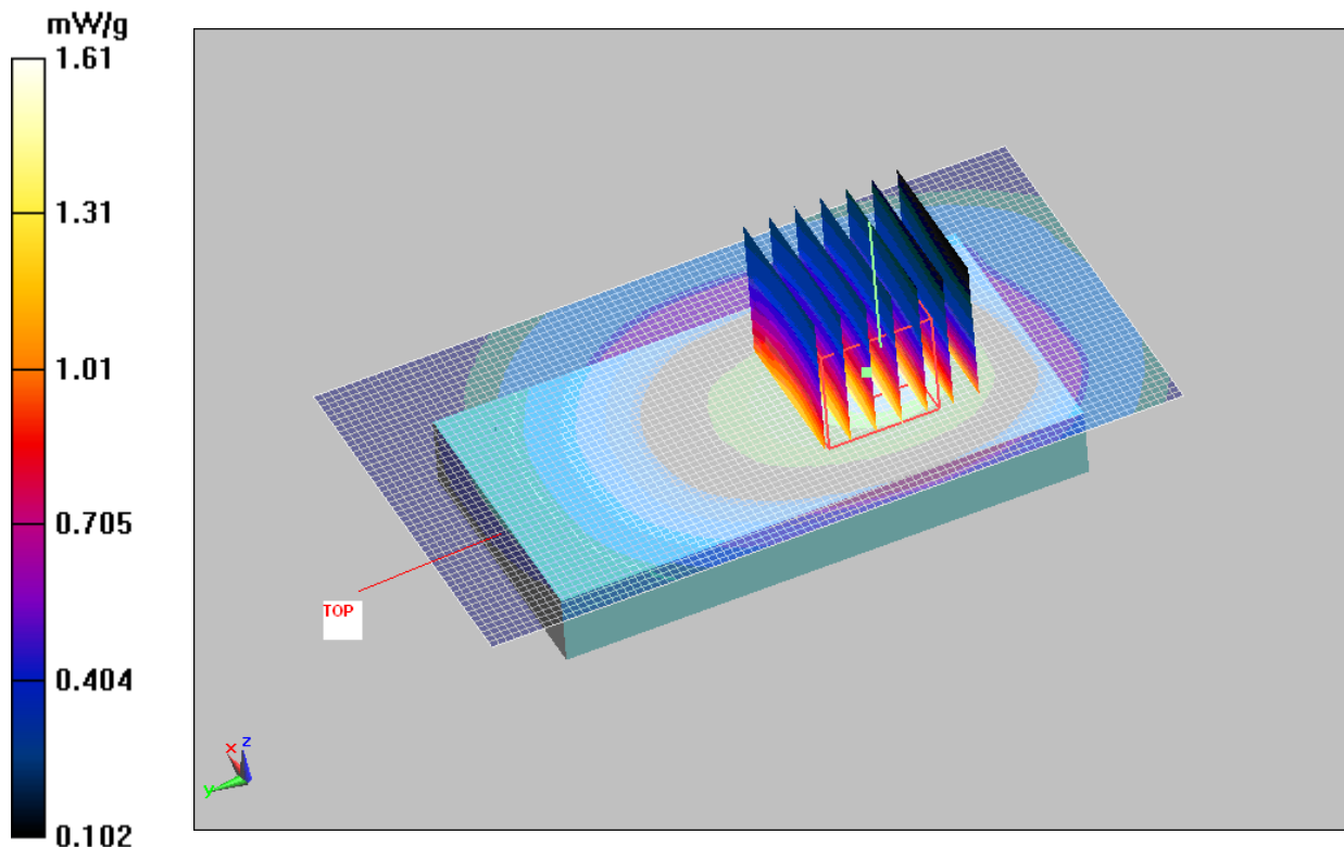
Figure 35 Body, Towards Ground, GSM 850 GPRS (4Up) Channel 251
