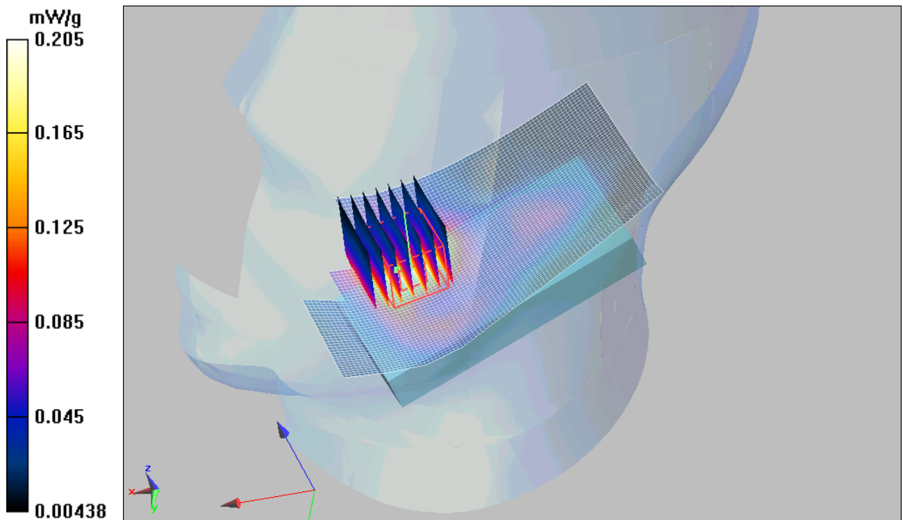
Figure 45 Right Hand Touch Cheek GSM 1900 Channel 661
