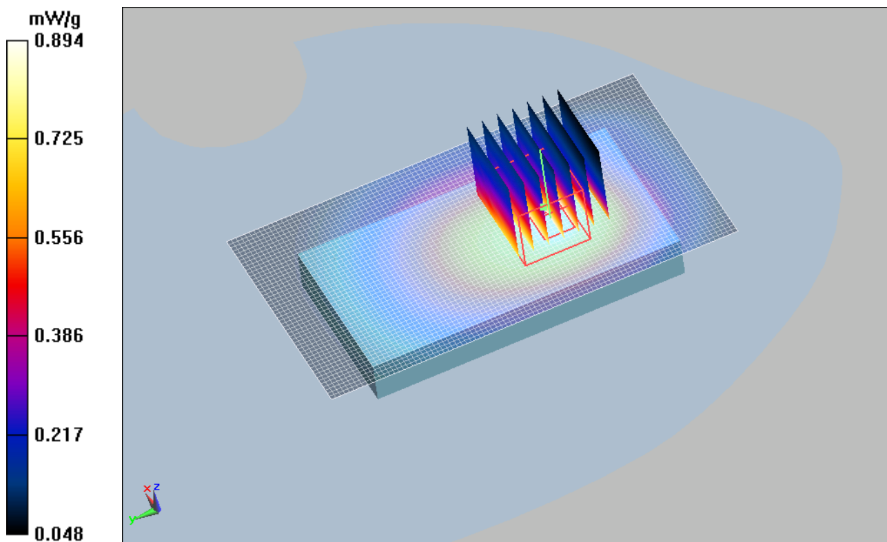
Figure 27 Body, Towards Ground, GSM 850 Channel 251
