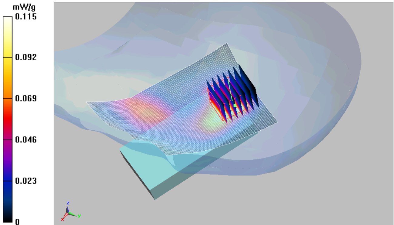
Figure 43 Left Hand Tilt 15^\circ GSM 1900 Channel 661
