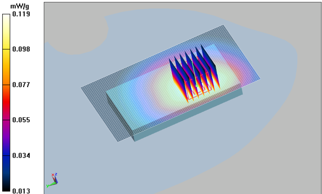
Figure 33 Body, Towards Phantom, GSM 850 Channel 190
