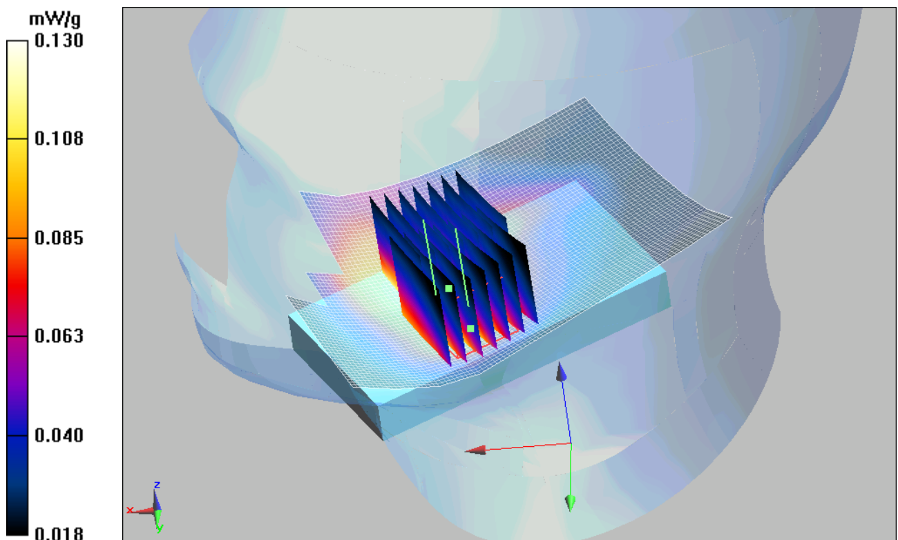
Figure 23 Right Hand Touch Cheek GSM 850 Channel 190
