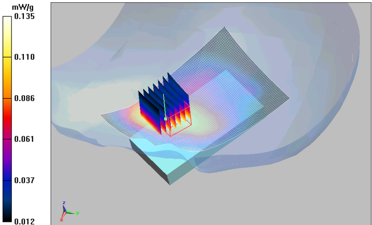
Figure 17 Left Hand Touch Cheek GSM 850 Channel 190
