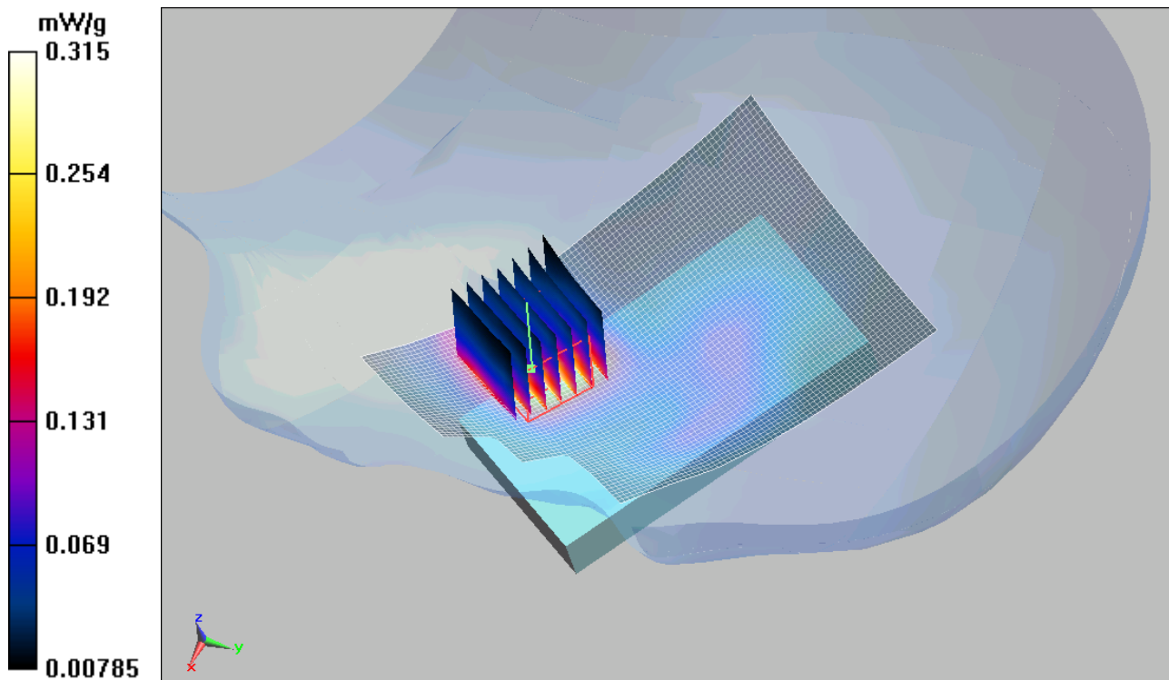
Figure 41 Left Hand Touch Cheek GSM 1900 Channel 512
