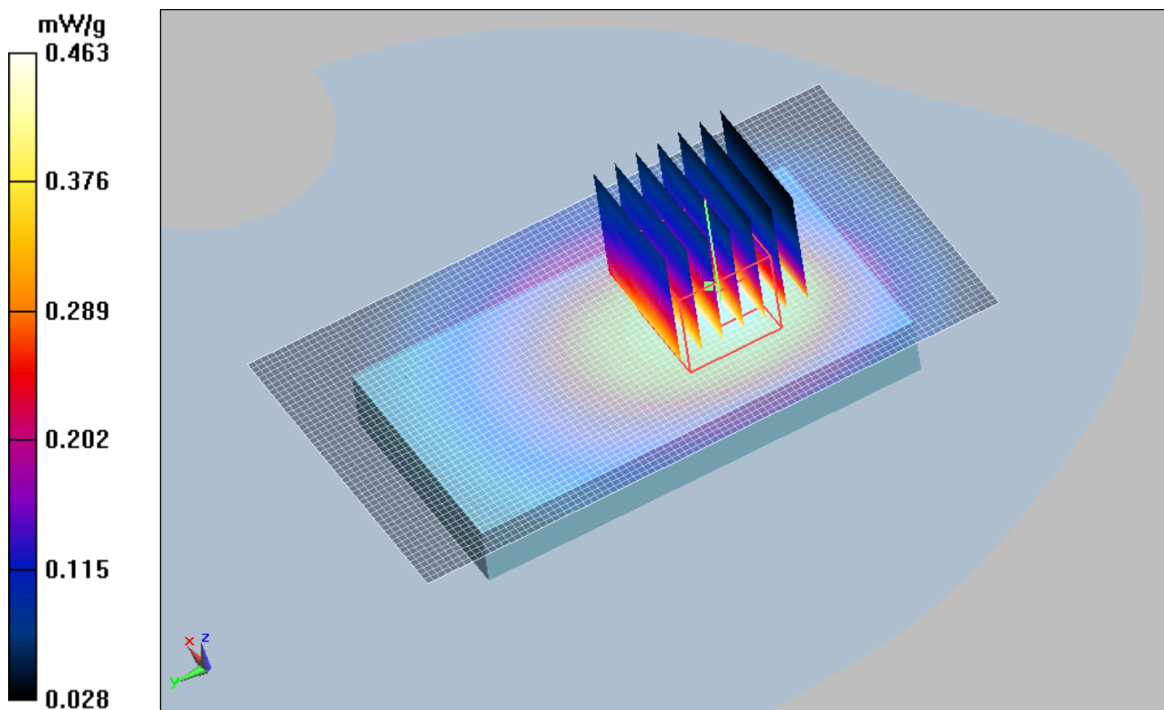
Figure 31 Body, Towards Ground, GSM 850 Channel 128
