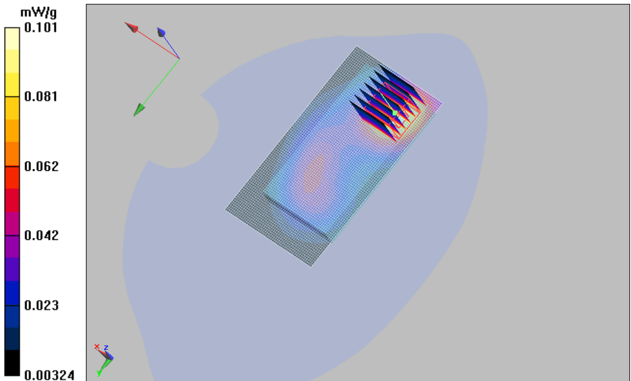
Figure 55 Body, Towards Phantom, GSM 1900 Channel 661
