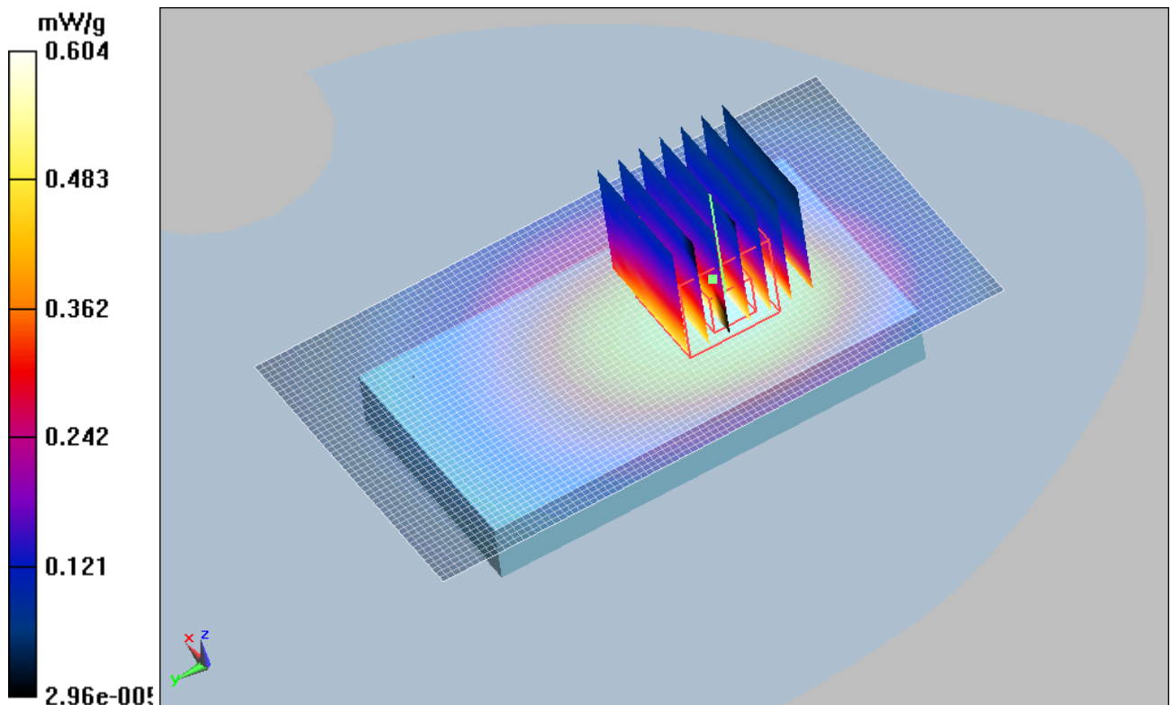
Figure 29 Body, Towards Ground, GSM 850 Channel 190
