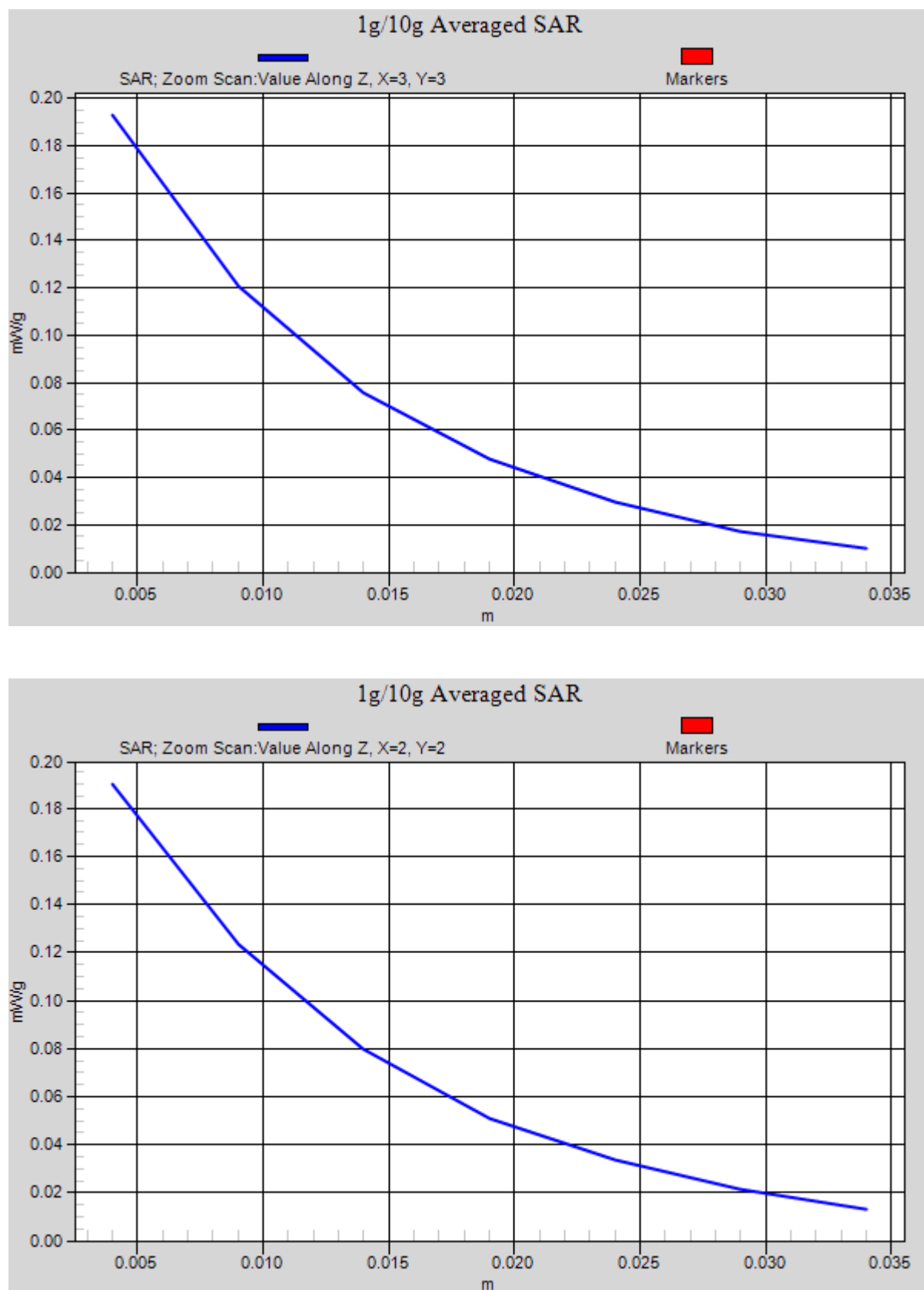
Figure 54 Z-Scan at power reference point (Body, Towards Ground, GSM 1900 Channel 512)
