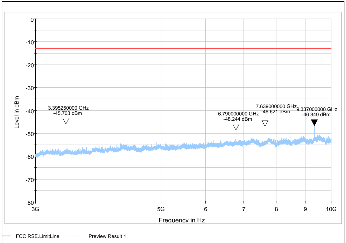
GSM 850 251 Channel 3GHz ~10GHz
