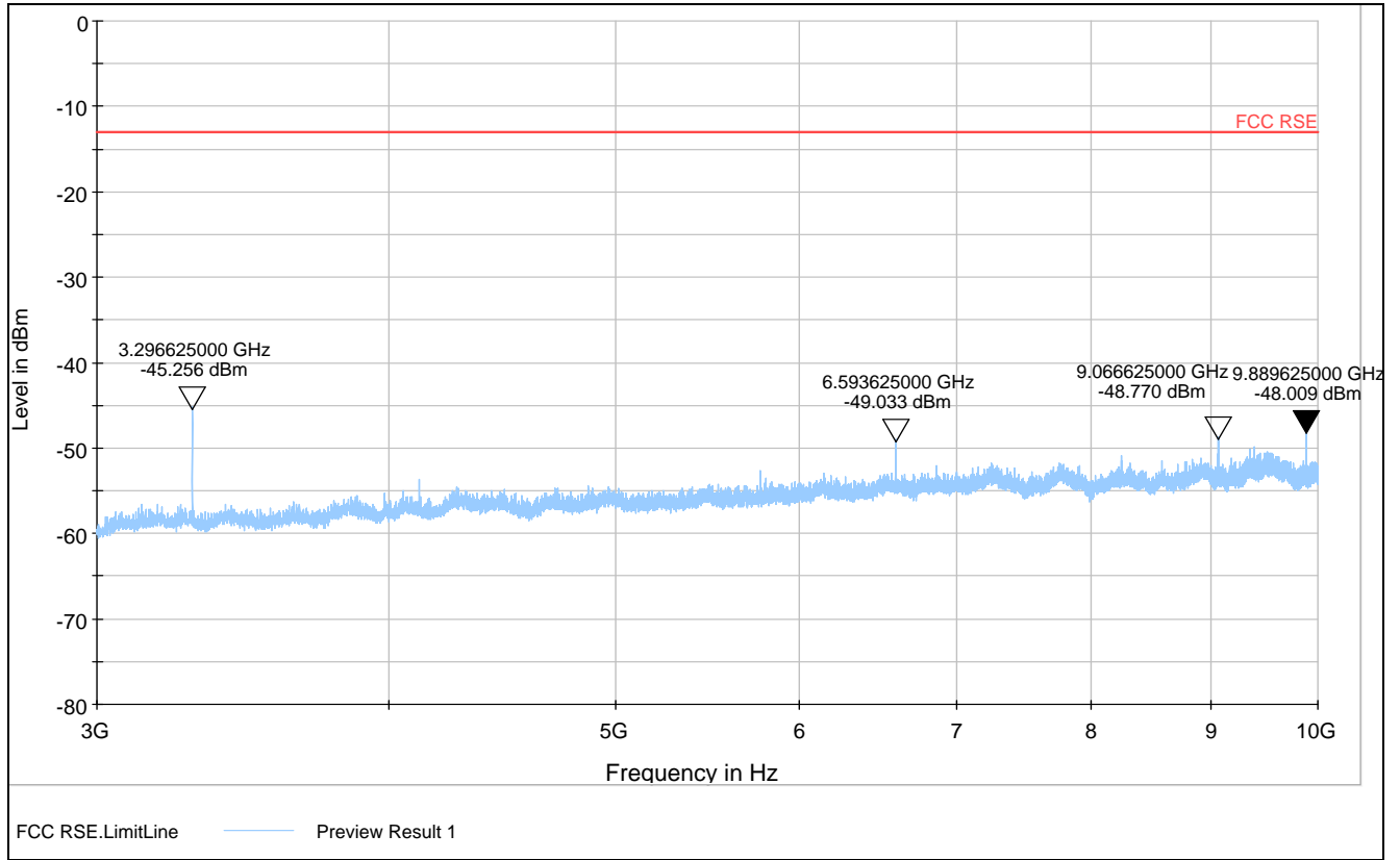
GSM 850 128 Channel 3GHz ~10GHz
