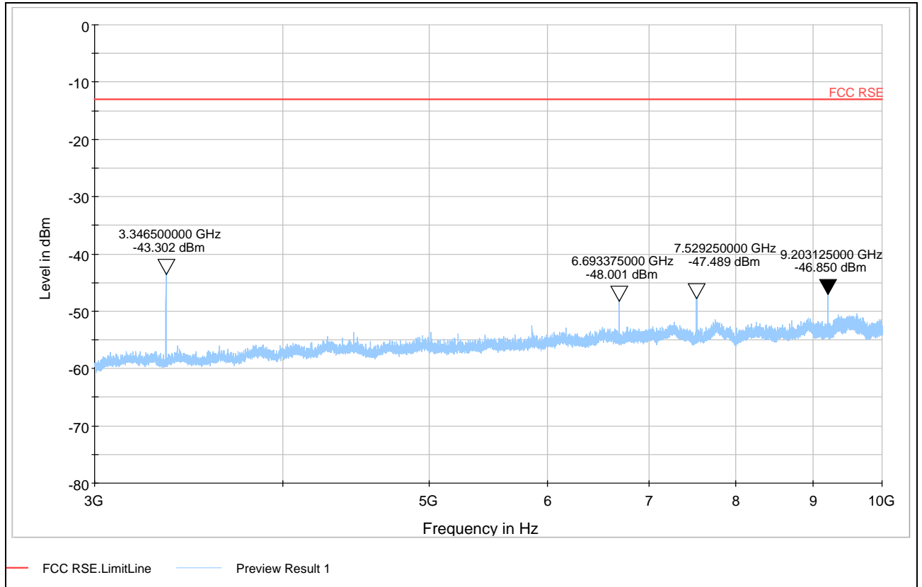
GSM 850 190 Channel 3GHz ~10GHz
