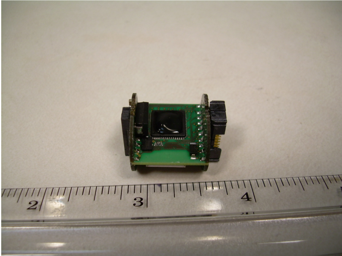
View of Side A of the PCB
