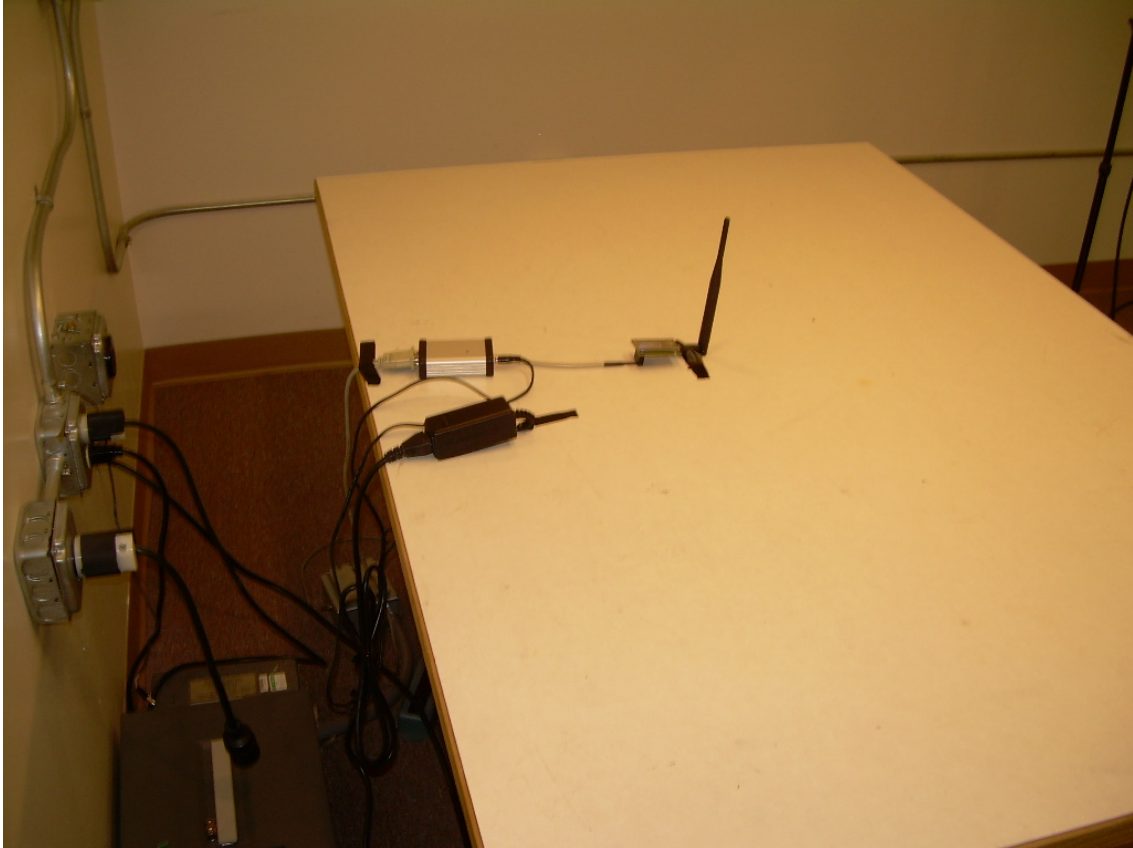
Photograph 5 - Back View Conducted Disturbance Worst Case Configuration
