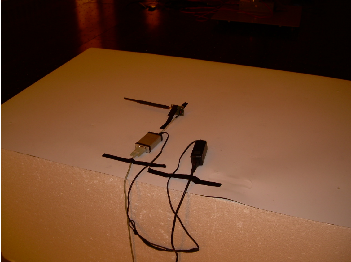
Photograph 2 - View Radiated Emissions in the Restricted Bands - On-Edge Orientation
