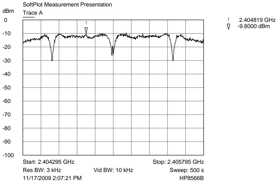
Trace A Lower channel 3kHz power spectral density
