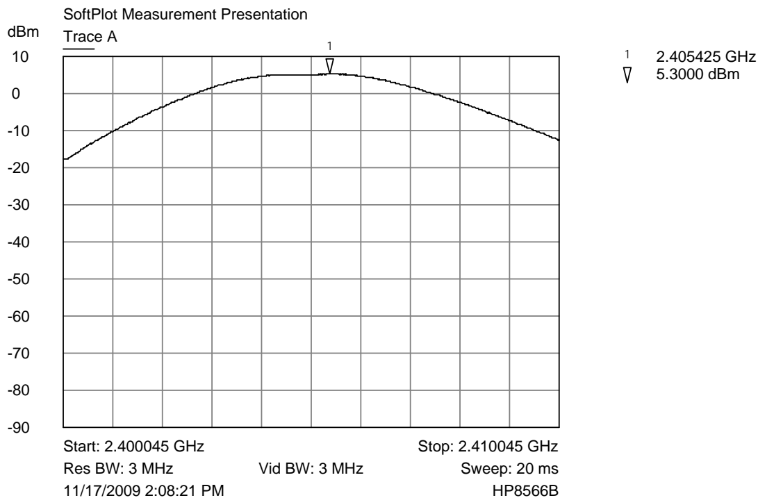
Trace A Lower channel output power
