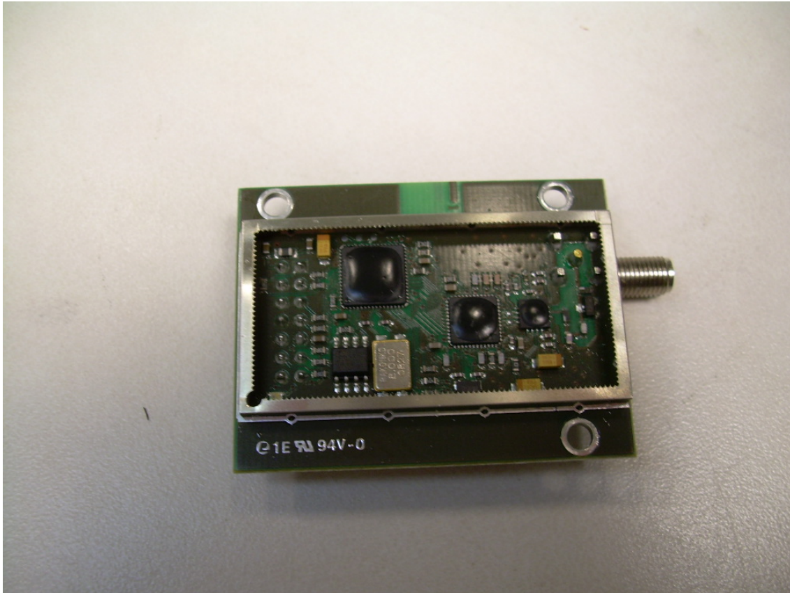
Photograph 7 - Front View of the EUT with RF Shielding Removed
