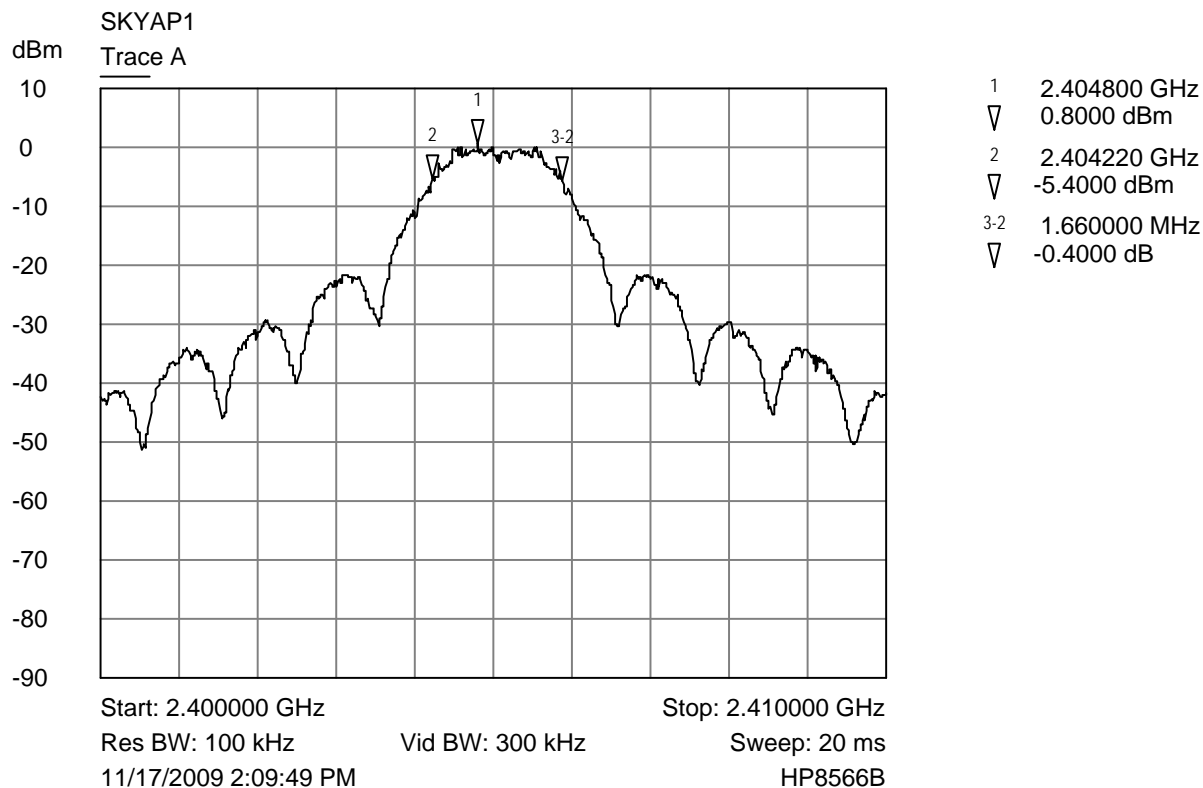
Trace A Lower channel band width
