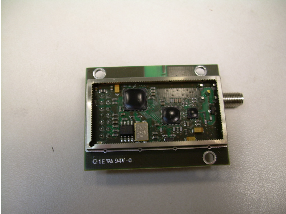
Front View of the EUT with RF Shielding Removed
