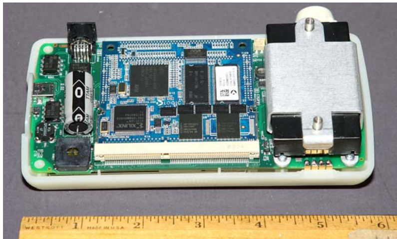
PC Board – Side 1c
