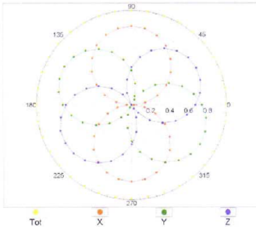
f=600 MHz,TEM
