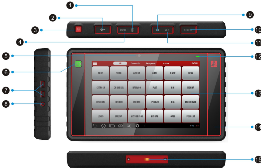
Fig. 2-4 X-431 PADII Tablet (front & side view)
