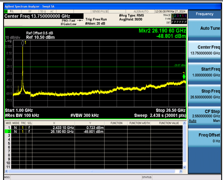
802.11n(HT40)_2437_0~Reference
