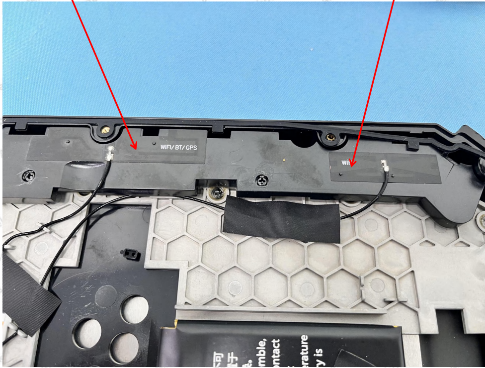
ANT 1 BT+WIFI+GNSS(RX)
