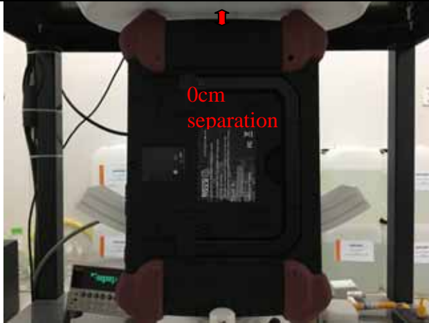
Body(Left Edge)
