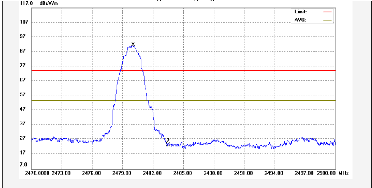
Pi/4 DQPSK Transmitting Band edge-right side Horizontal
