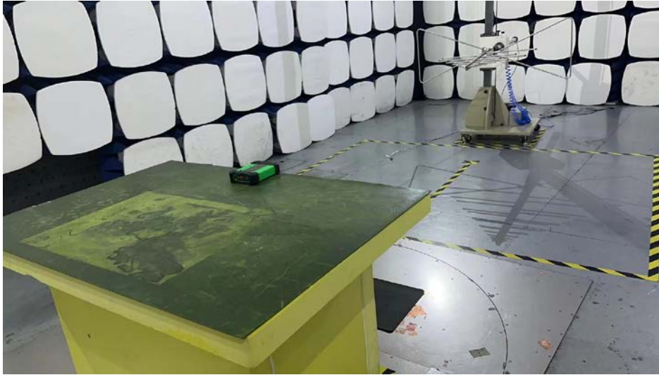
Spurious Emission Test Setup (Above 1GHz)
