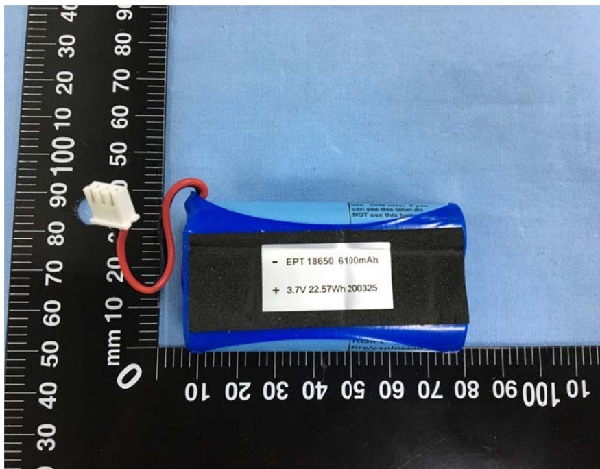
Battery View
