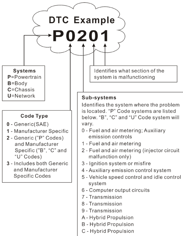
Figure 2-1 (P0201 - Injector circuit malfunction, Cylinder 1)
