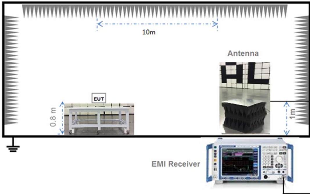
For Radiated Emission Test (Below 30 MHz))
