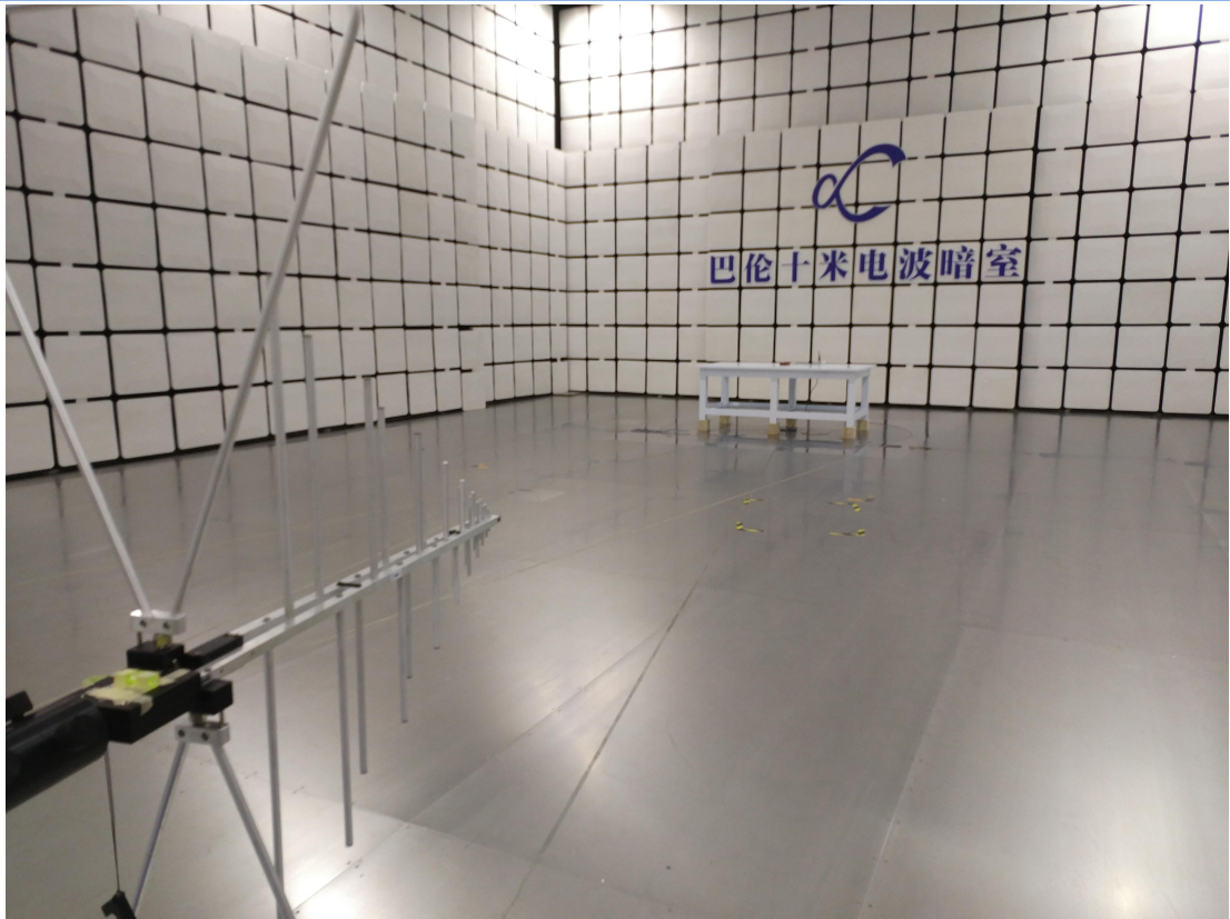
30 MHz-1 GHz
