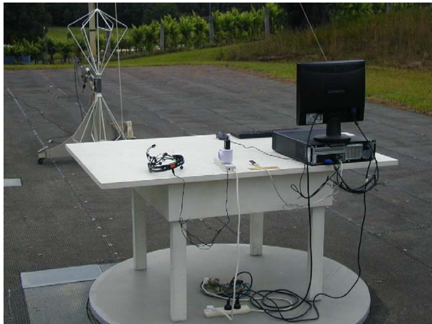
FCC Part 15B Radiated Disturbance Test Setup (Rear View – EUT Charging Mode)
