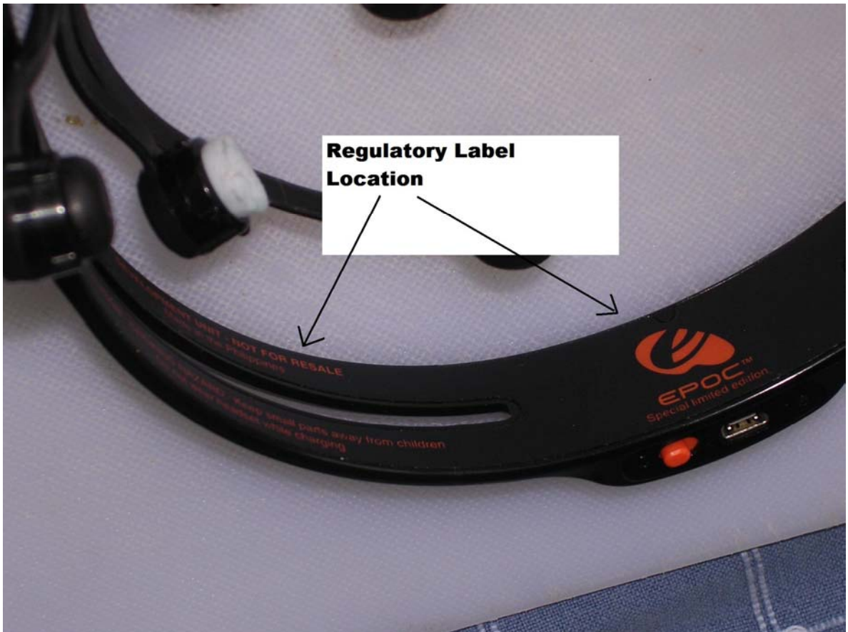
FCC Label Location on EUT
