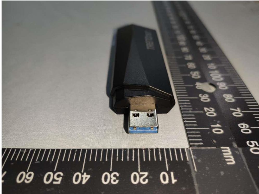
Outview: TEW-905UB Pic 6
