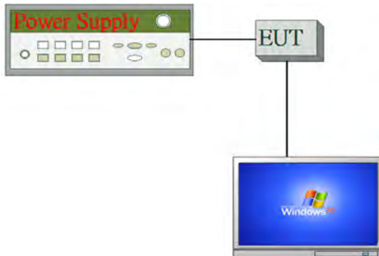
Fig. 2-2 Conducted Emission
