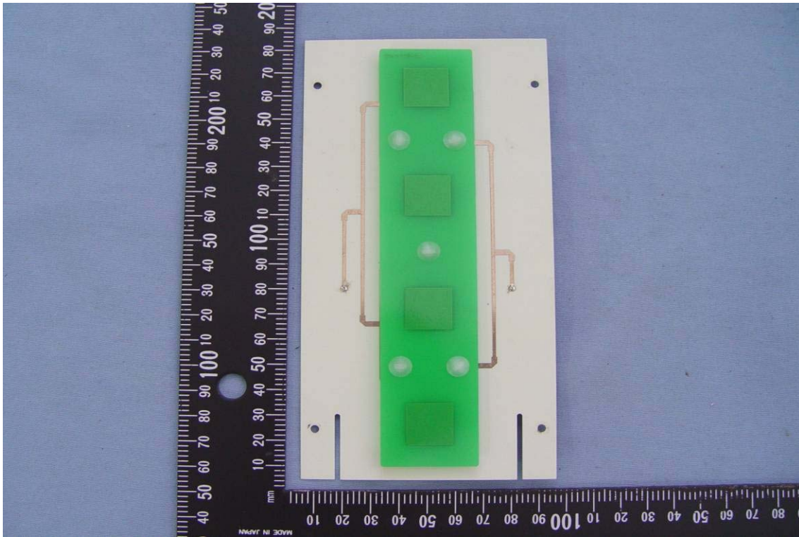
Patch Antenna
