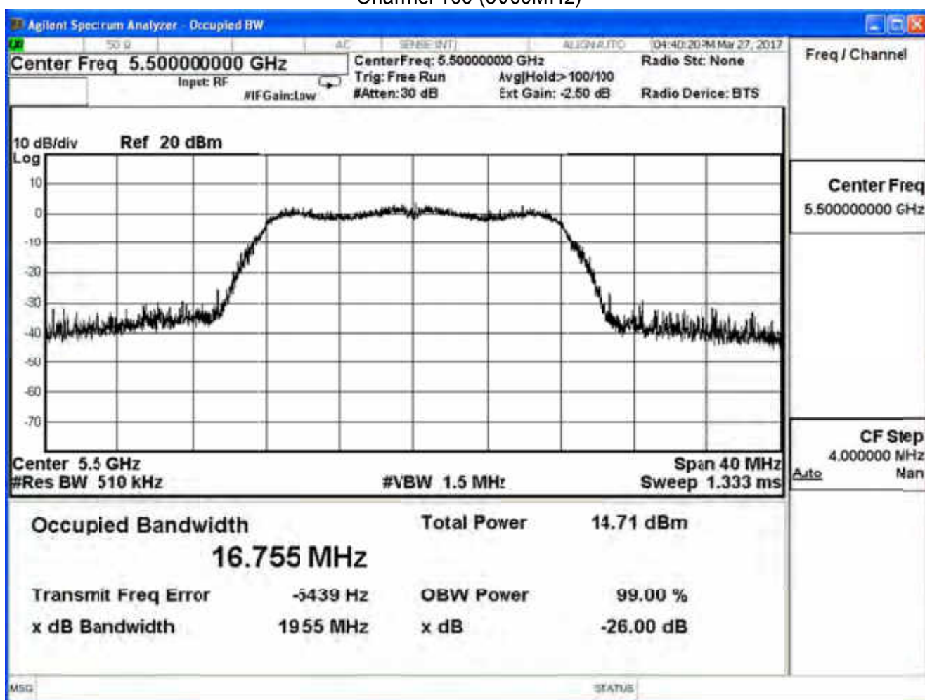
Channel 100 (5500MHz)
