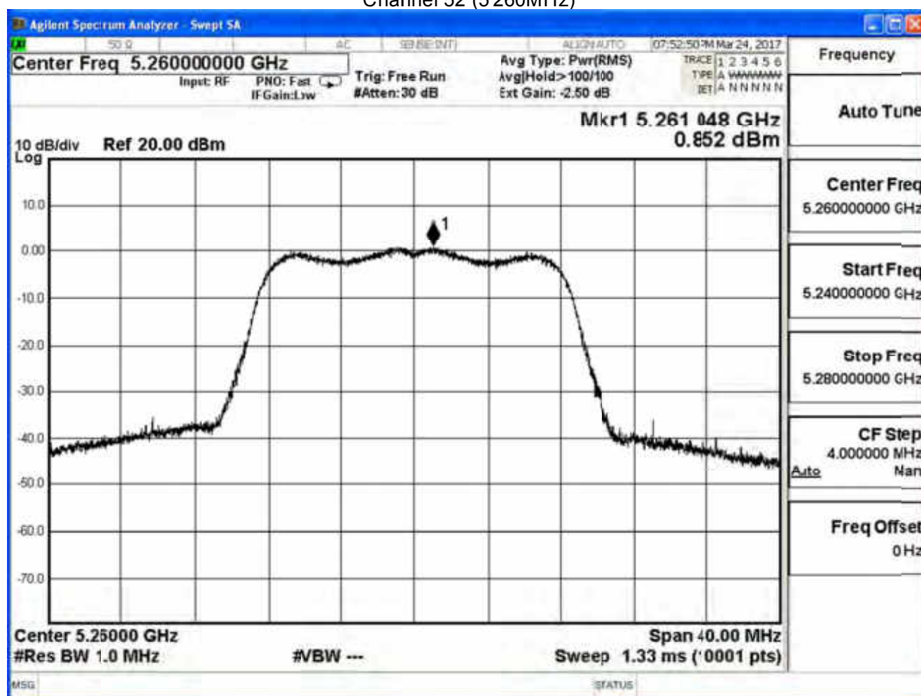
Channel 52 (5 260MHz)
