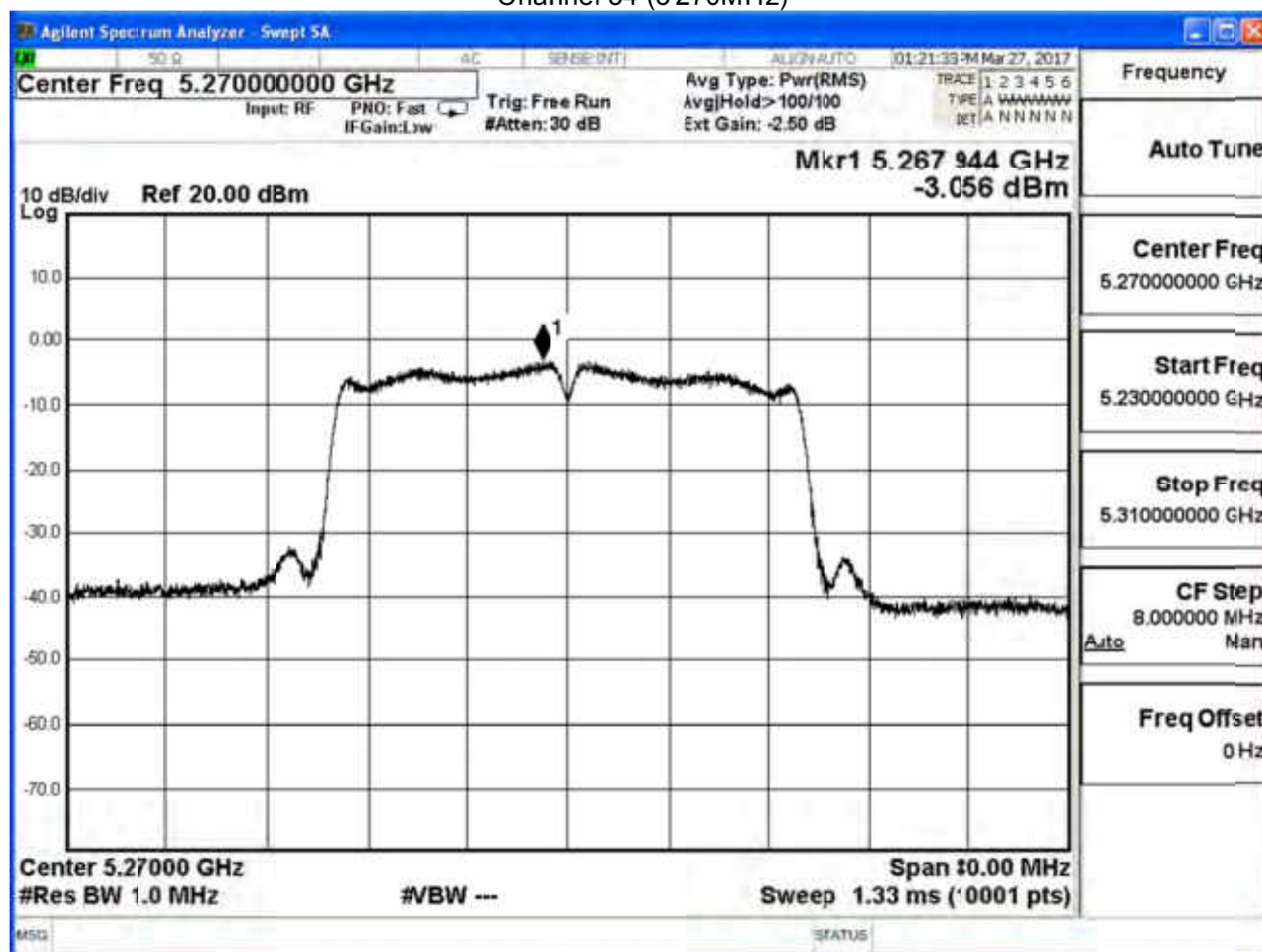
Channel 54 (5 270MHz)
