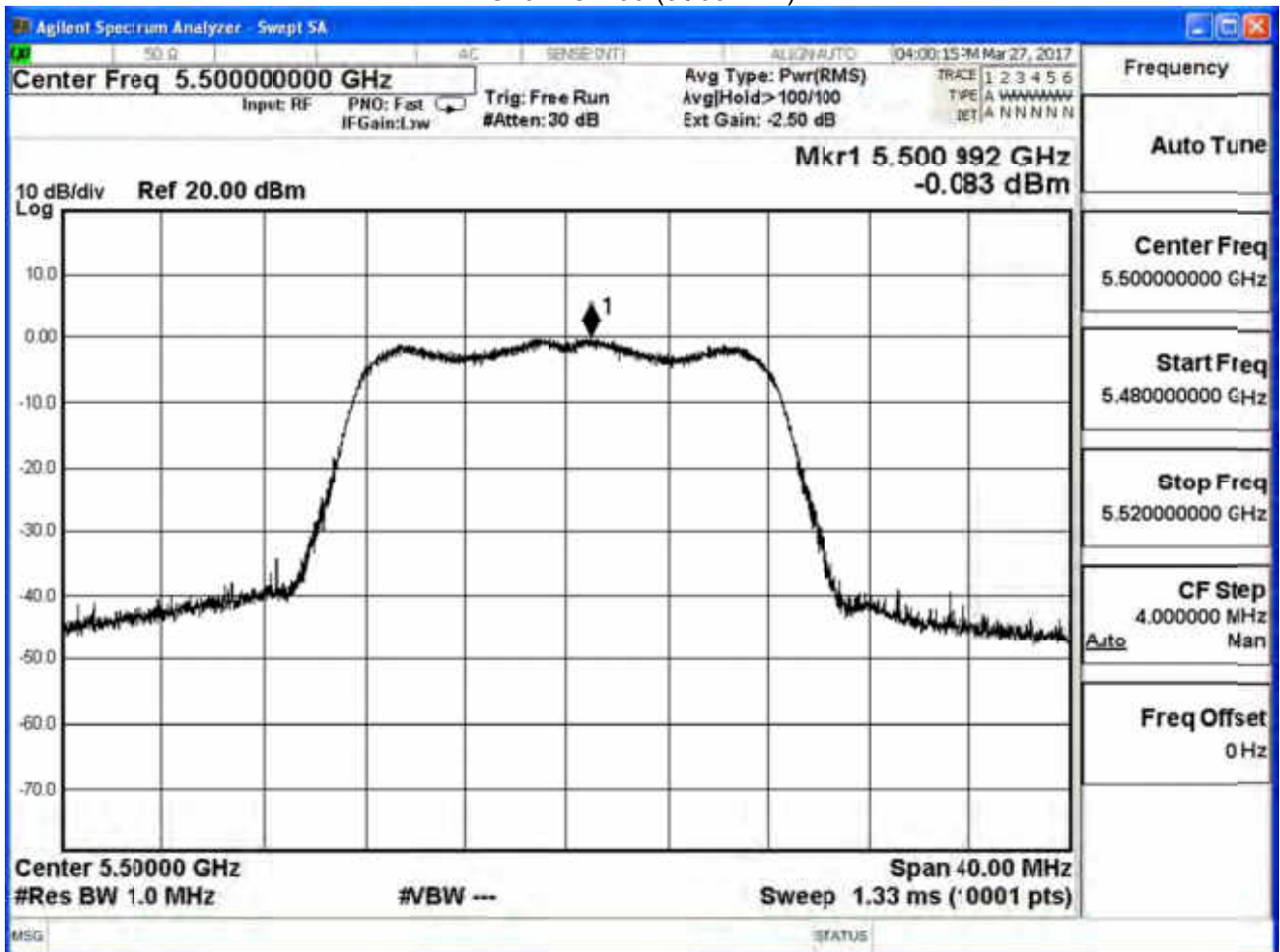
Channel 100 (5500MHz)
