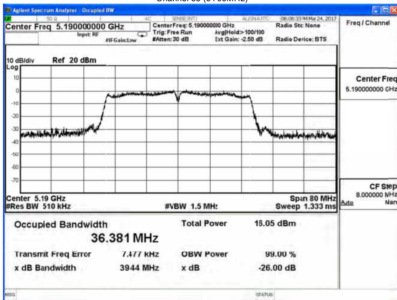
Channel 38 (5190MHz)
