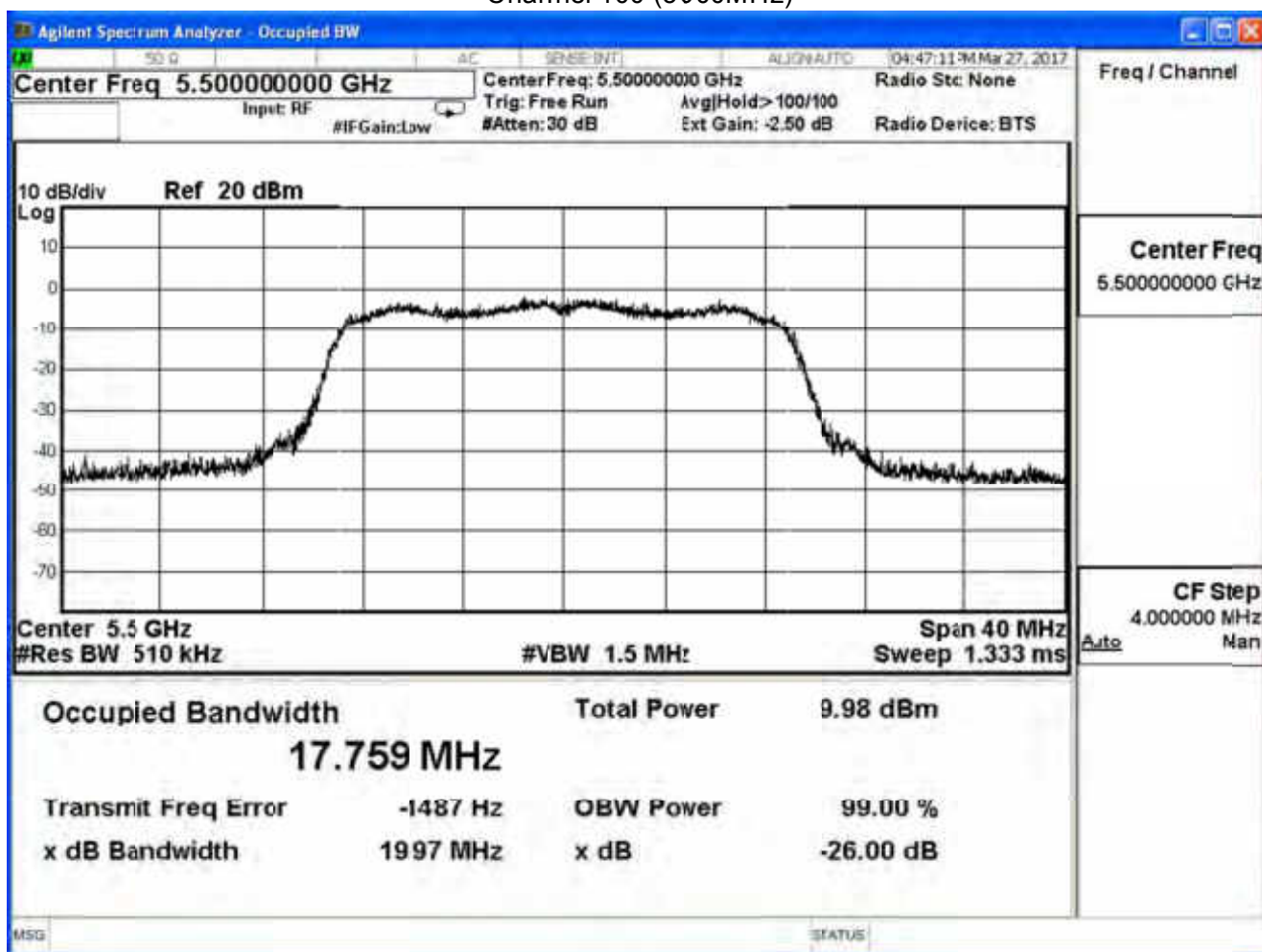
Channel 100 (5500MHz)
