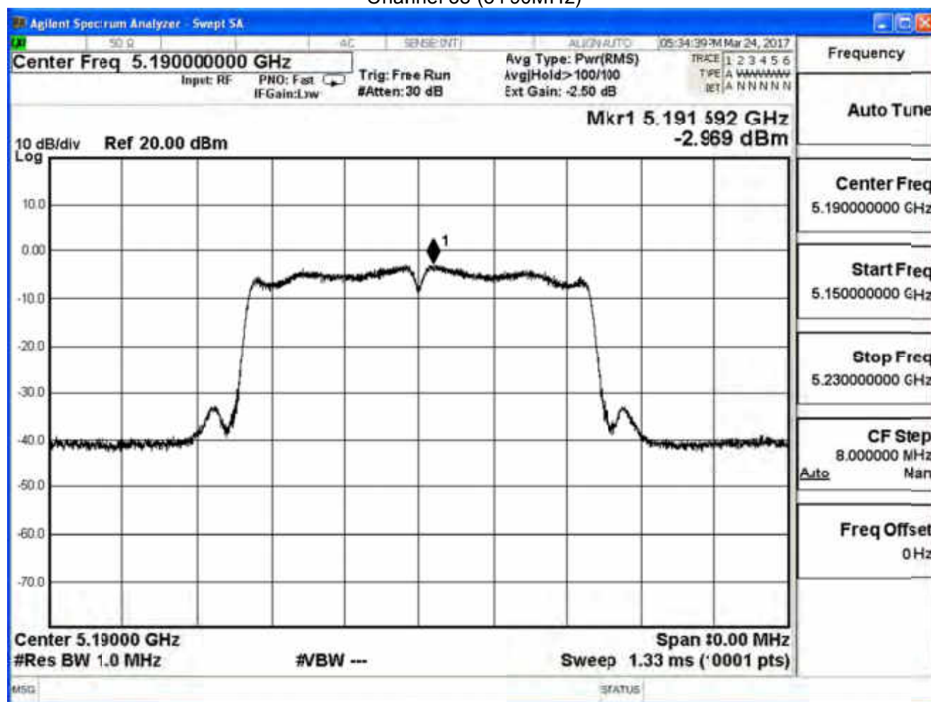
Channel 38 (5190MHz)
