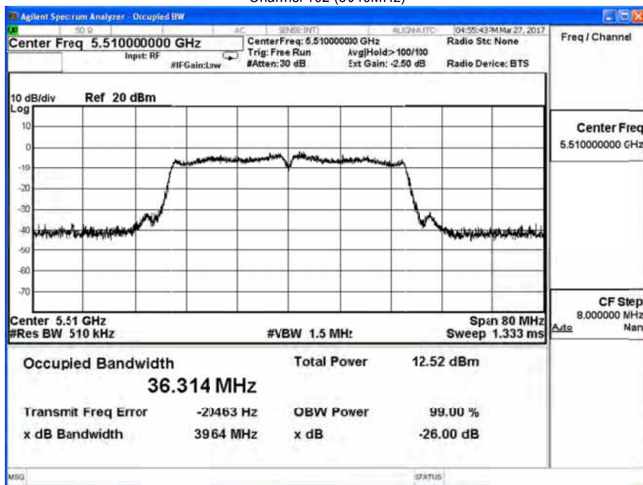
Channel 102 (5510MHz)
