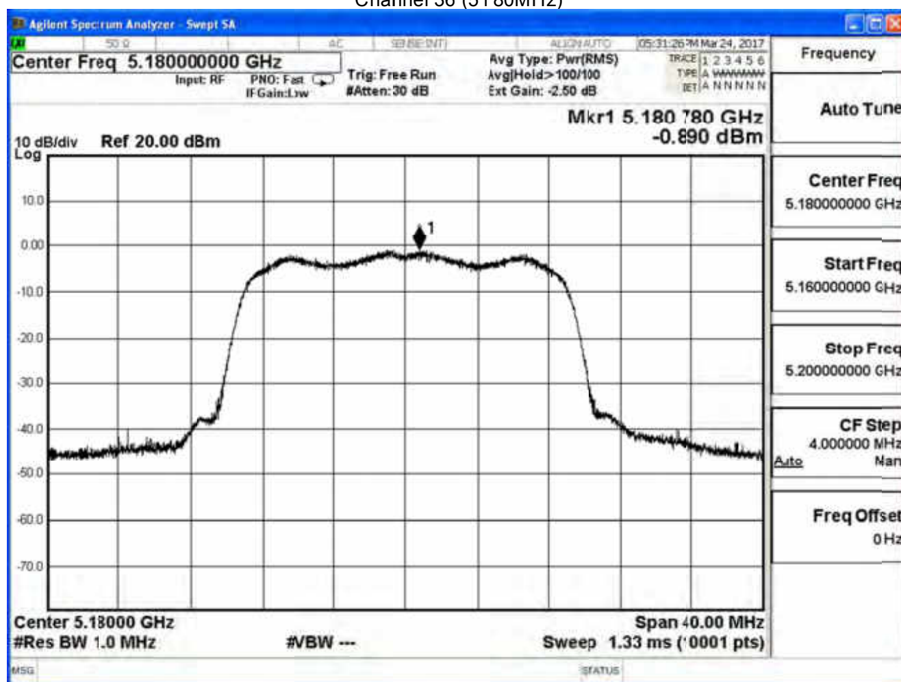
Channel 36 (5180MHz)
