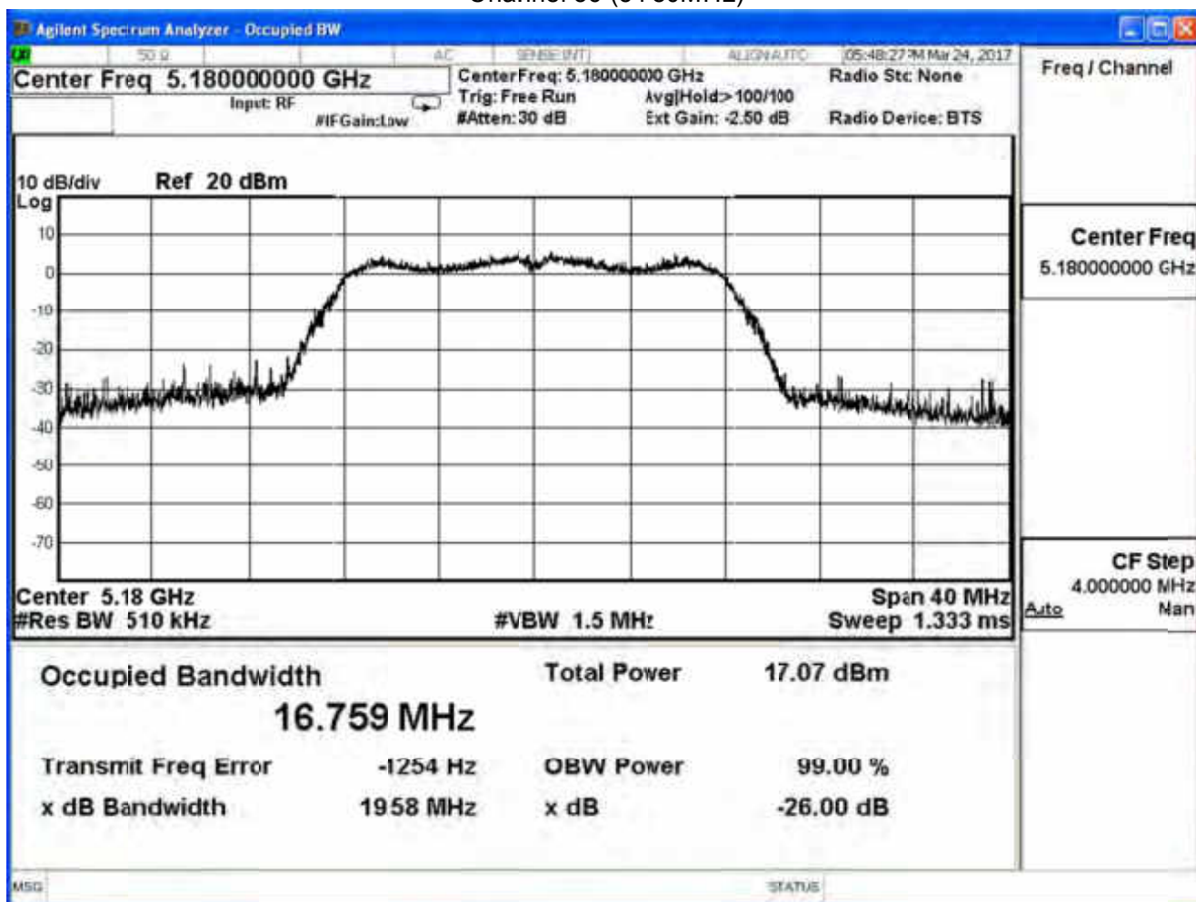
Channel 36 (5180MHz)
