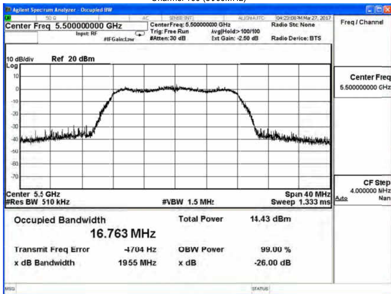
Channel 100 (5500MHz)
