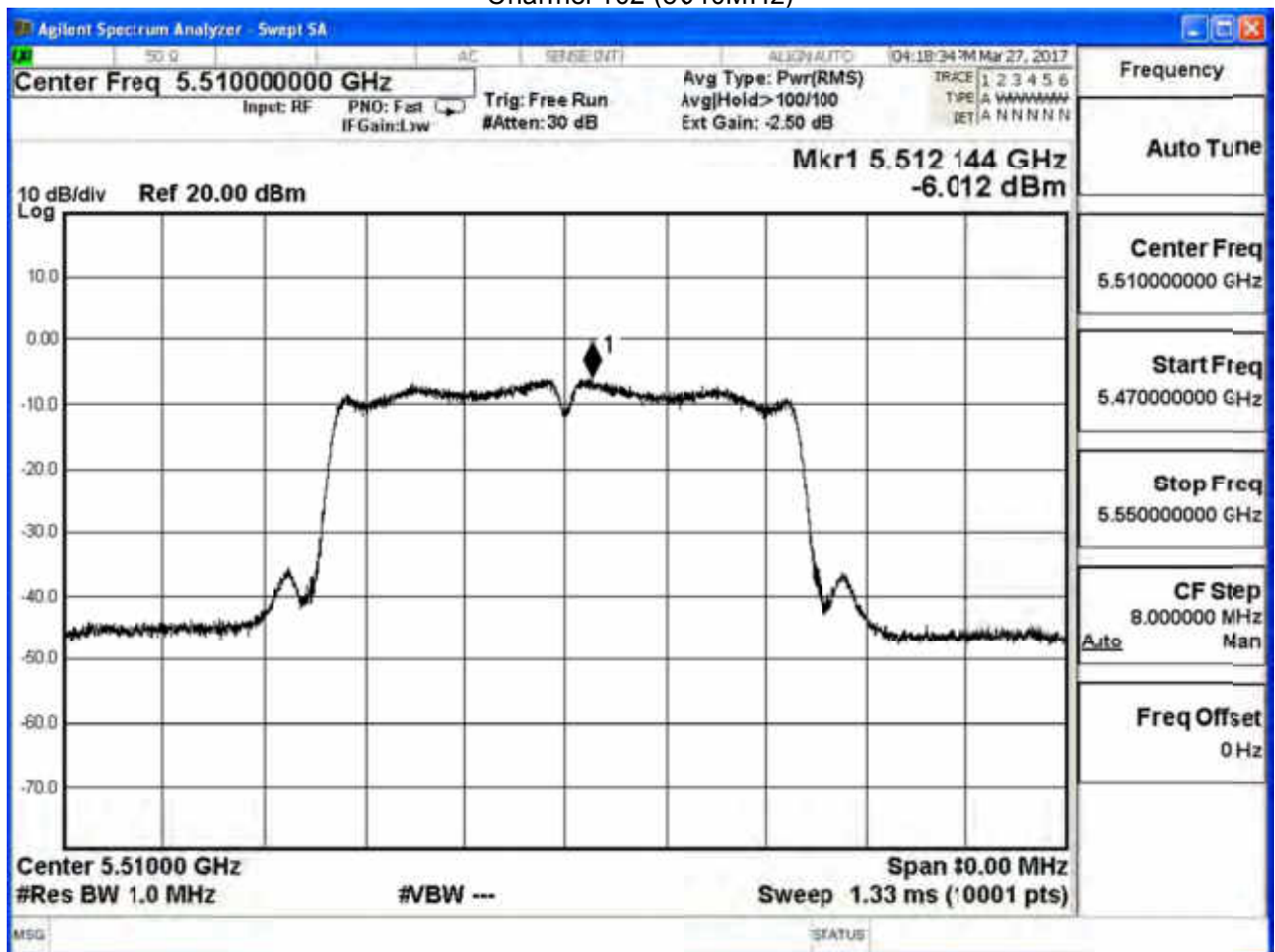
Channel 102 (5510MHz)
