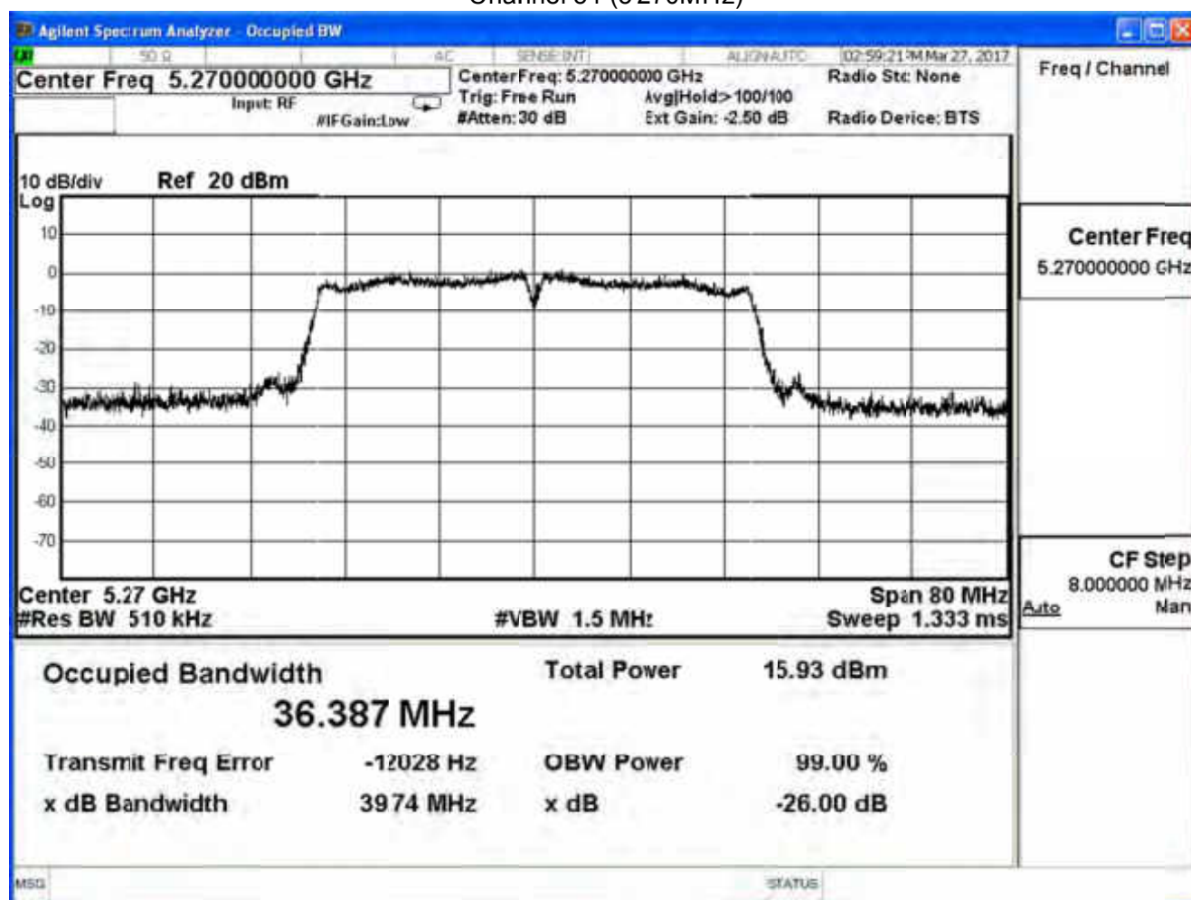
Channel 54 (5 270MHz)
