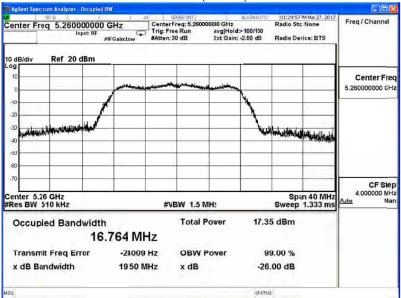
Channel 52 (5 260MHz)
