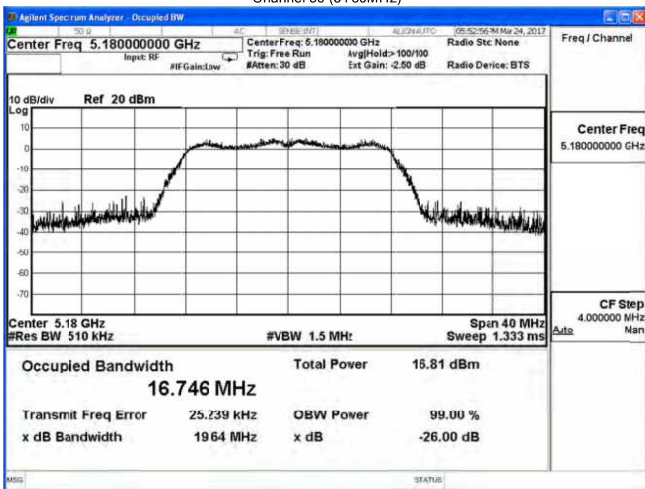
Channel 36 (5180MHz)
