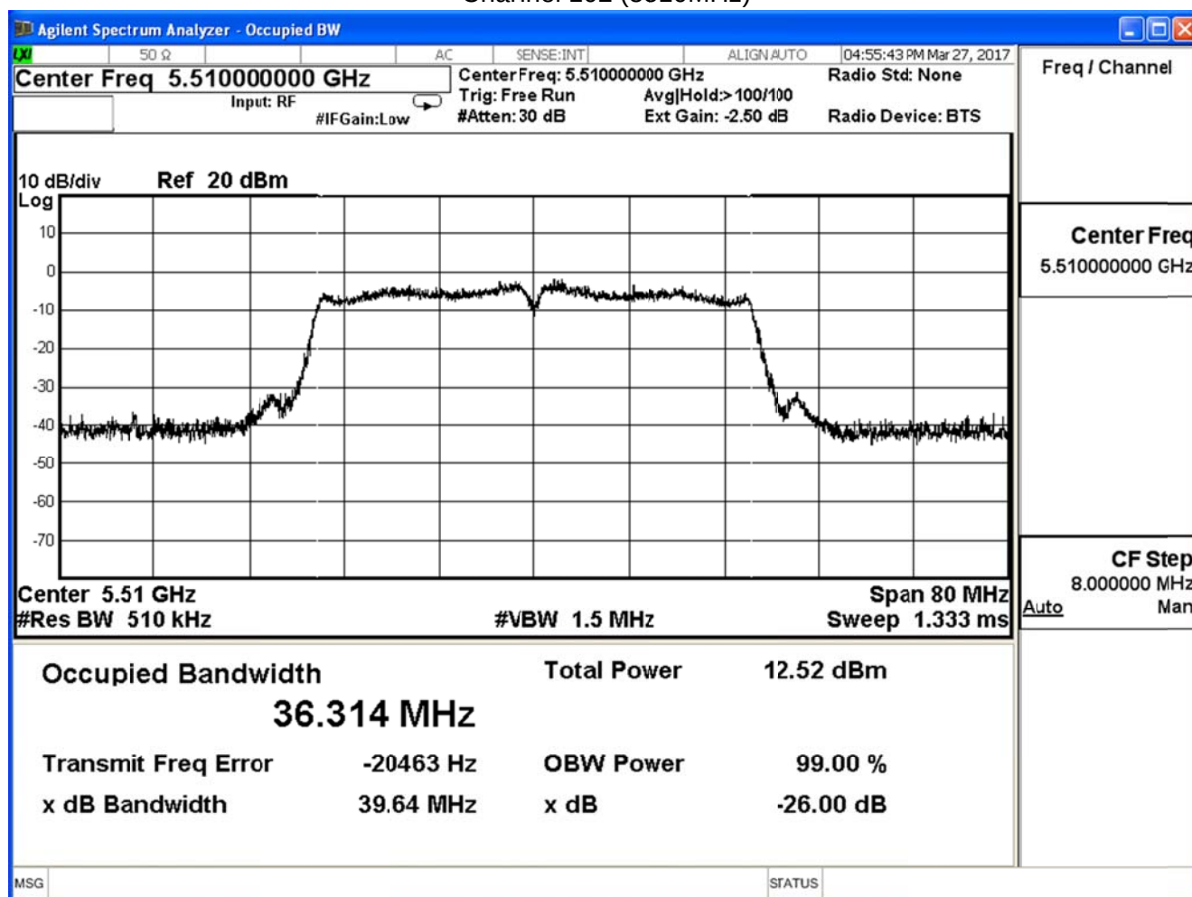
Channel 102 (5510MHz)
