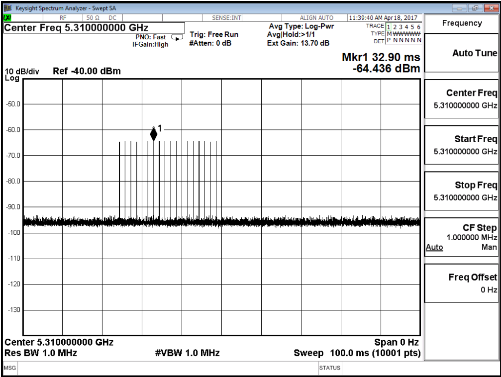
Radar Type 0 Calibration Plot (5310MHz)
