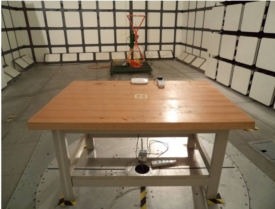
Below 1GHz Radiated Emissions – Front View (adapter Power)
