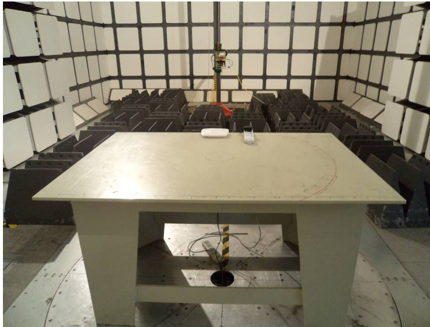
Above 1GHz Radiated Emissions – Front View (adapter Power)
