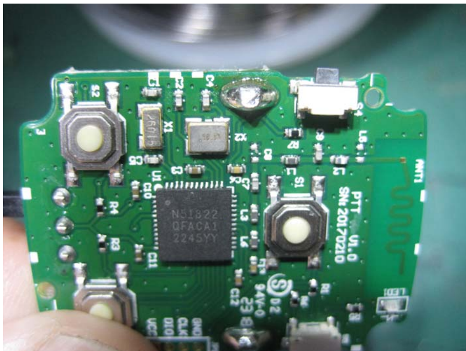
Closer View of BT module & Printed Trace Antenna
