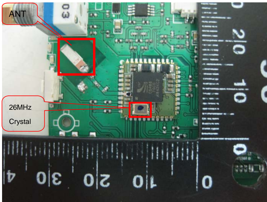
Closer View of the Bluetooth module
