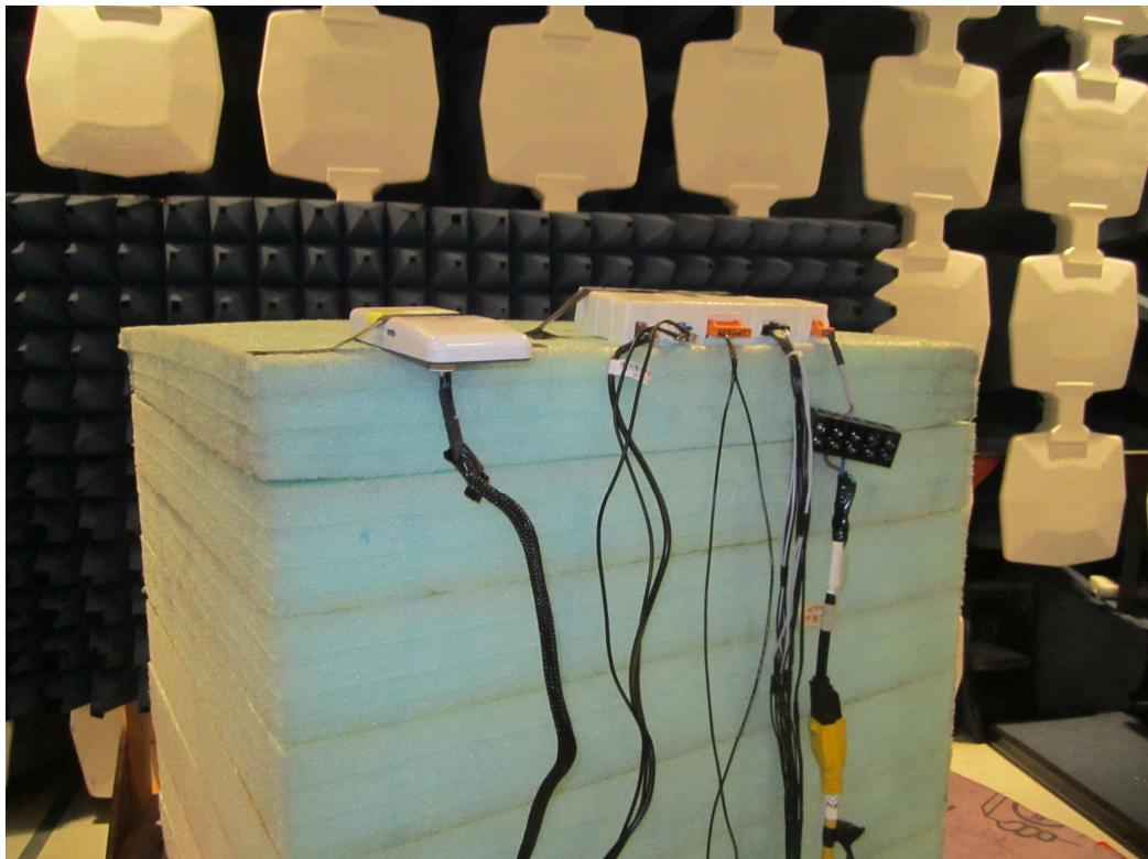
Z Orientation
