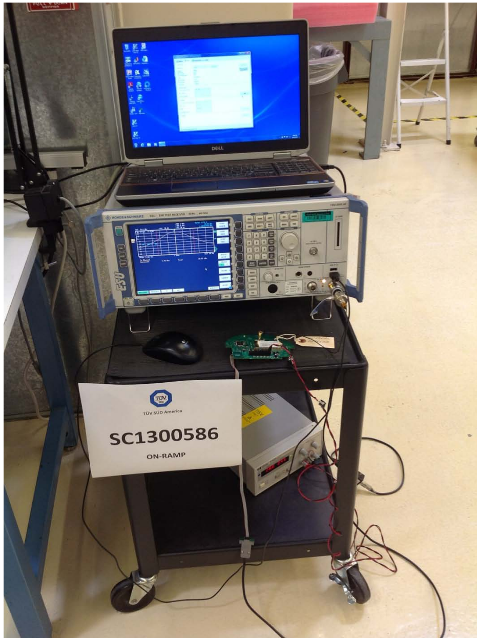
Conducted Port measurements
