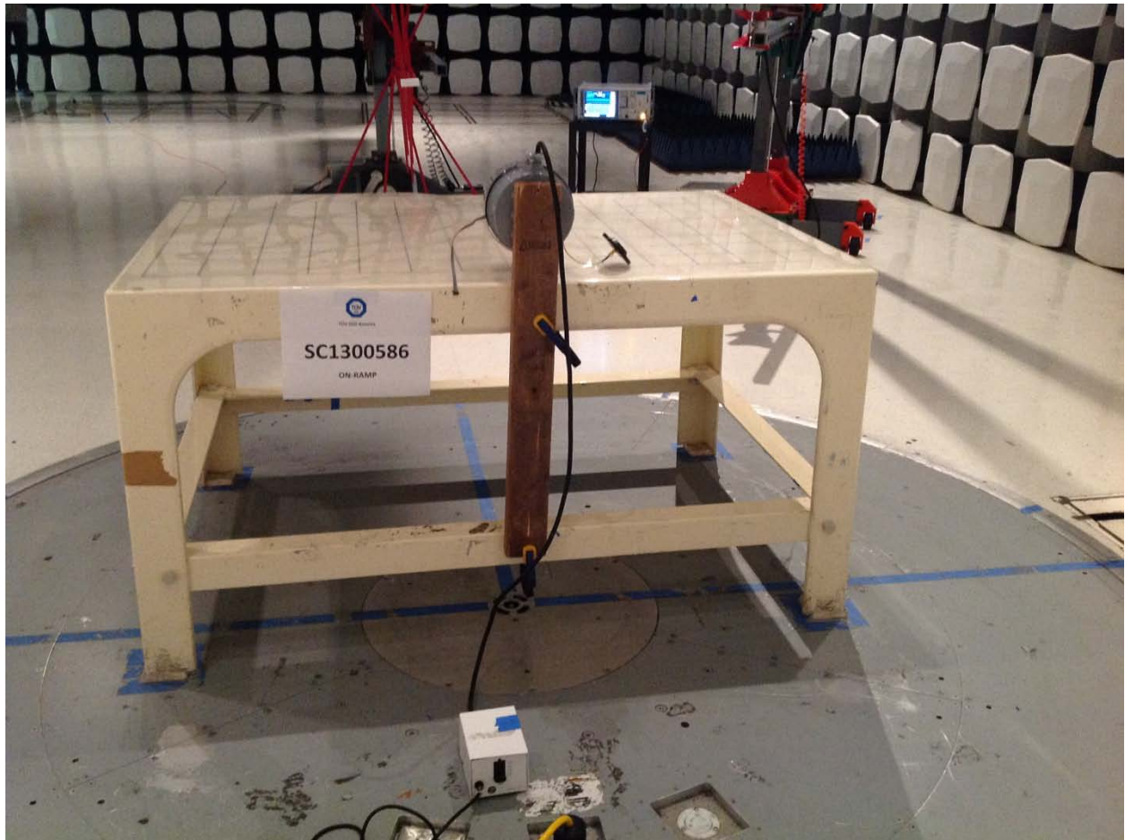
Radiated Emissions (Back Side)
