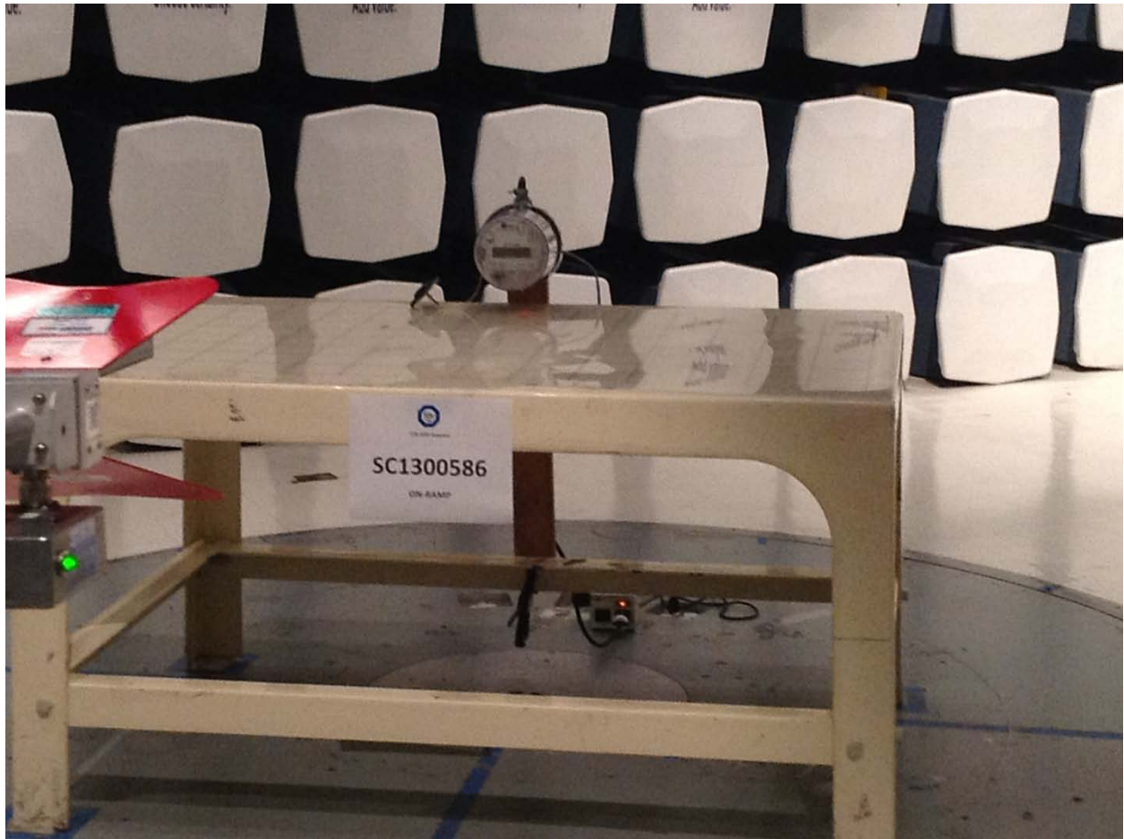
Above 1 GHz (Radiated Emissions)
