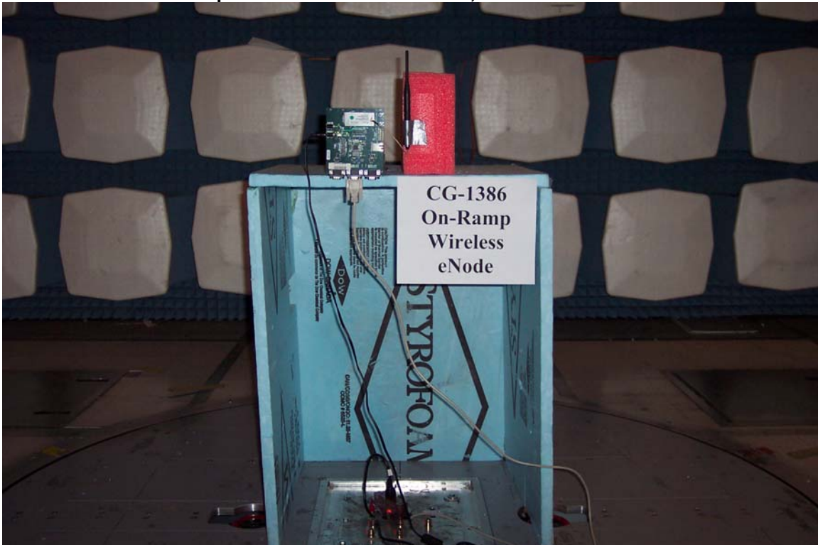
Radiated Emission setup with 5dBi Antenna vertical, EUT Vertical
