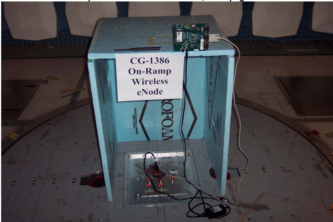
Radiated Emission setup with 5dBi Antenna Horizontal, EUT Upright
