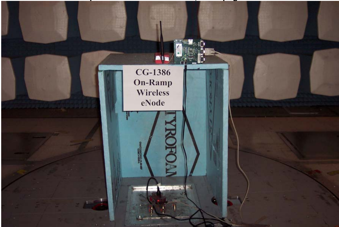
Radiated Emission setup with 5dBi Antenna vertical, EUT Upright
