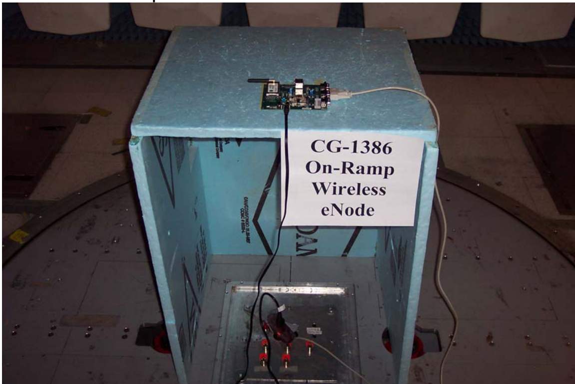
Radiated Emission setup with 1dBi Antenna Horizontal
