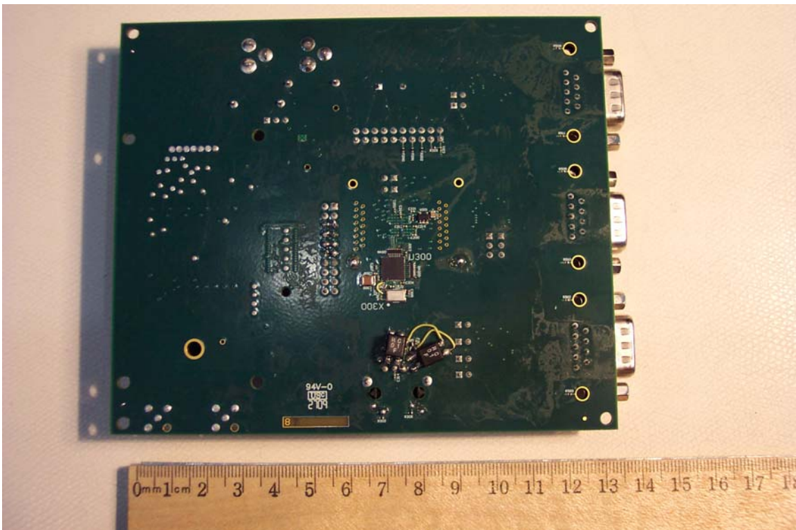
Rear view of developer board
