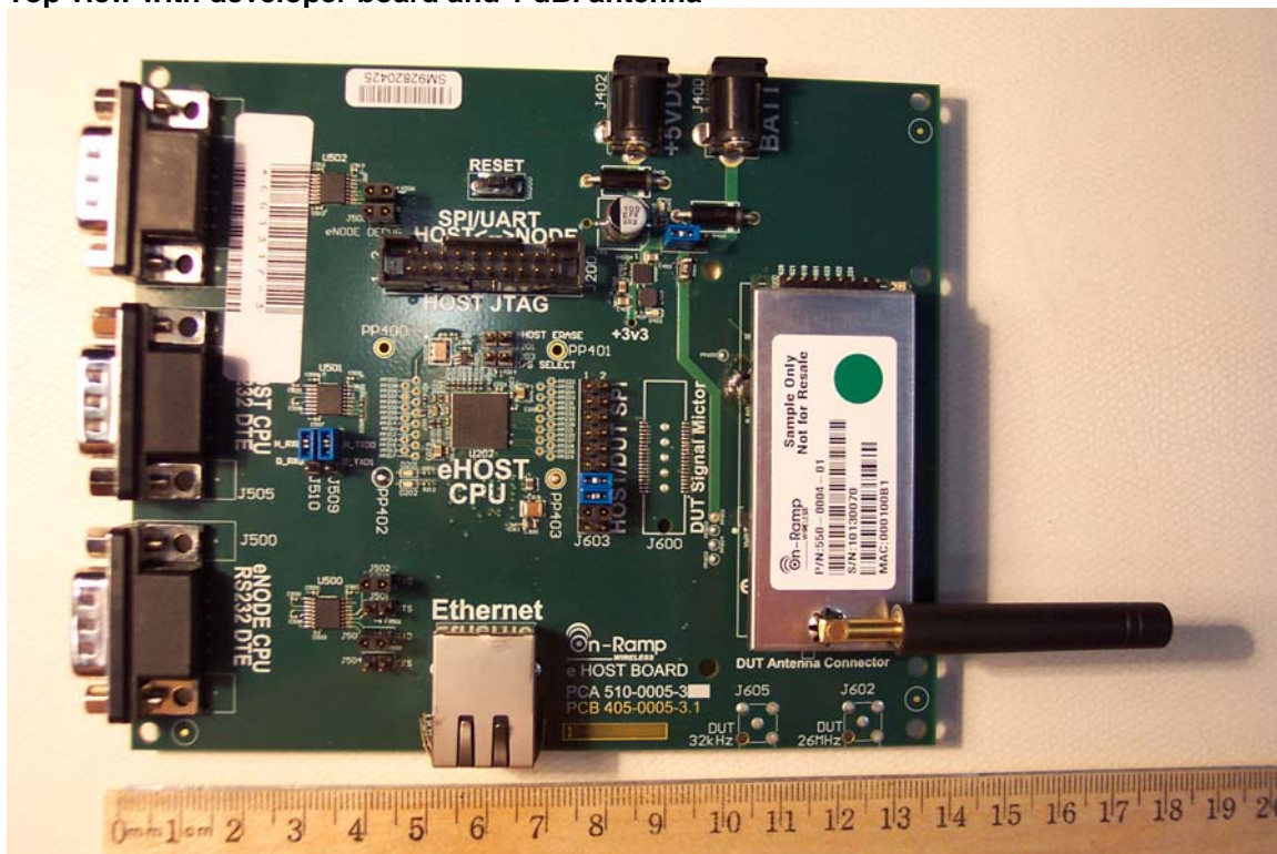
Top view with developer board and 2 dBi antenna
