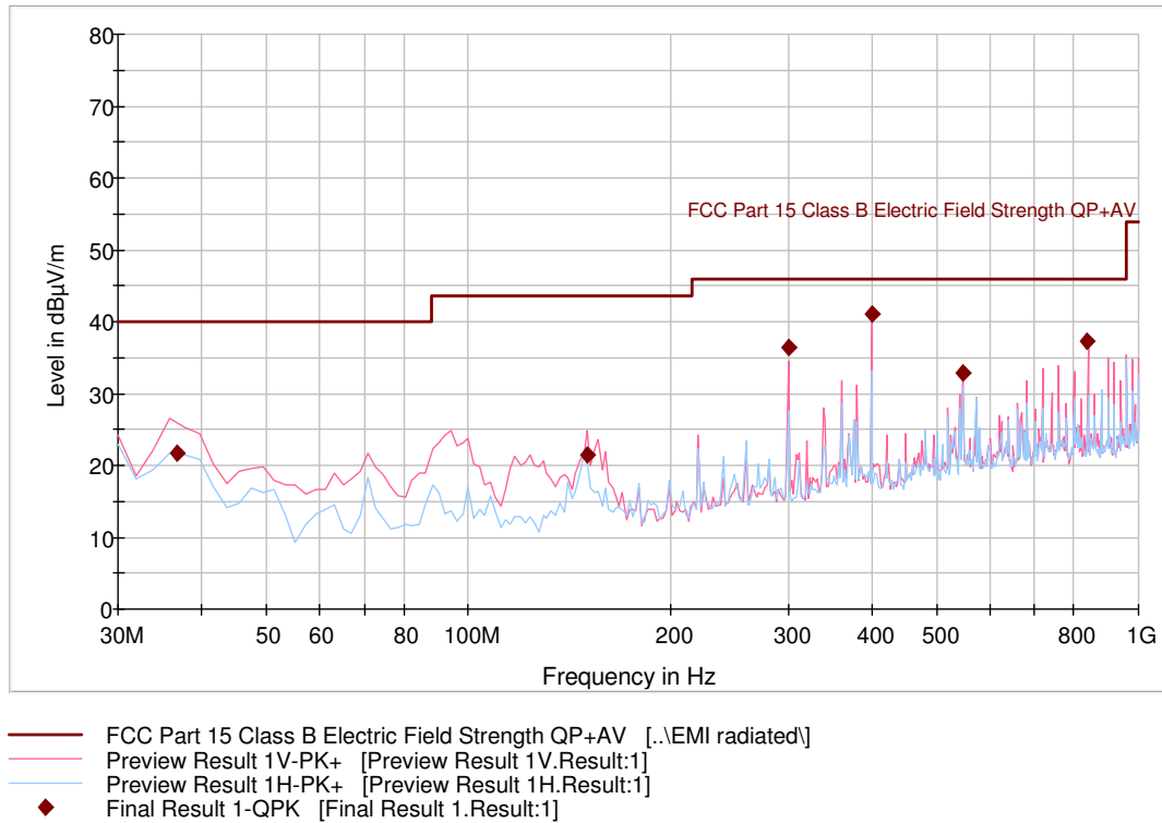
TUV 3m Radiated 30 to 1000MHz
